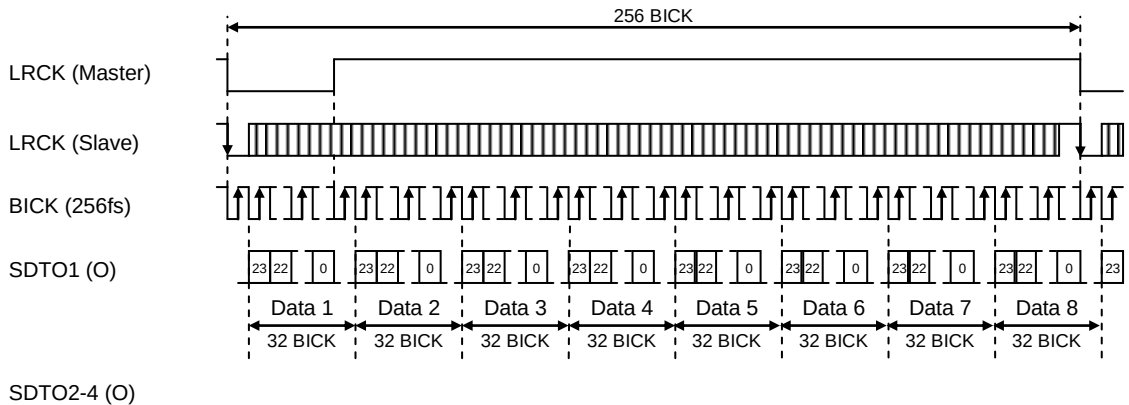
Figure 47. Mode 33/37 Timing (TDM256 Mode, I²S Compatible, 24-bit)
