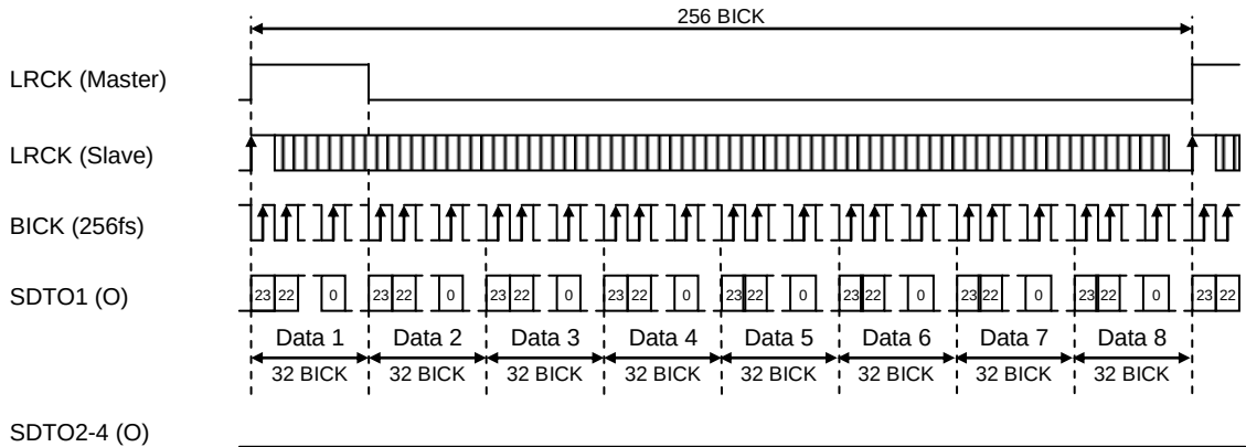
Figure 46. Mode 32/36 Timing (TDM256 Mode, MSB Justified, 24-bit)
