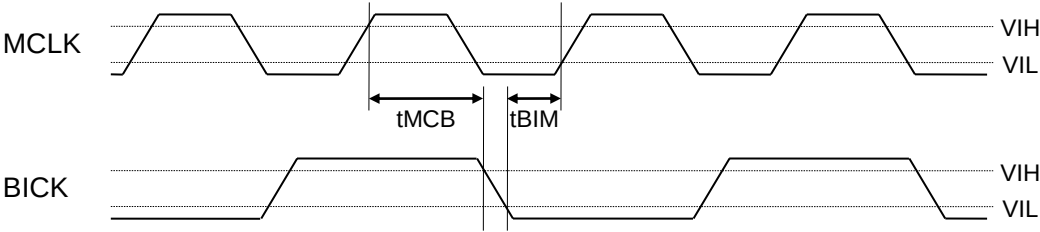
Figure 54. Audio Interface Timing (Slave mode, TDM mode, MCLK=2 \times BICK )
