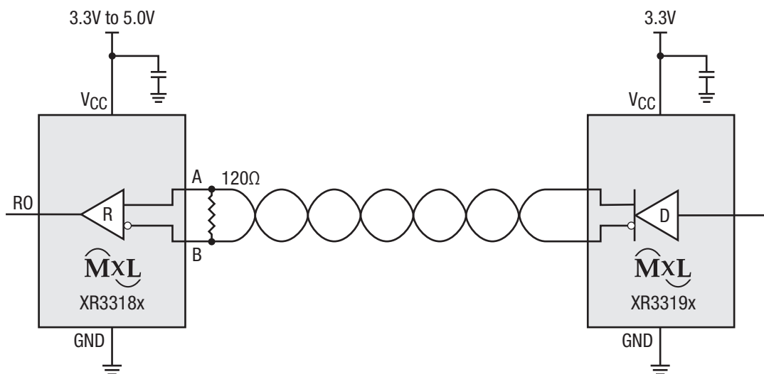
Figure 1. Typical Application
