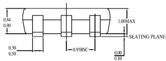
SIDE VIEW - 2
