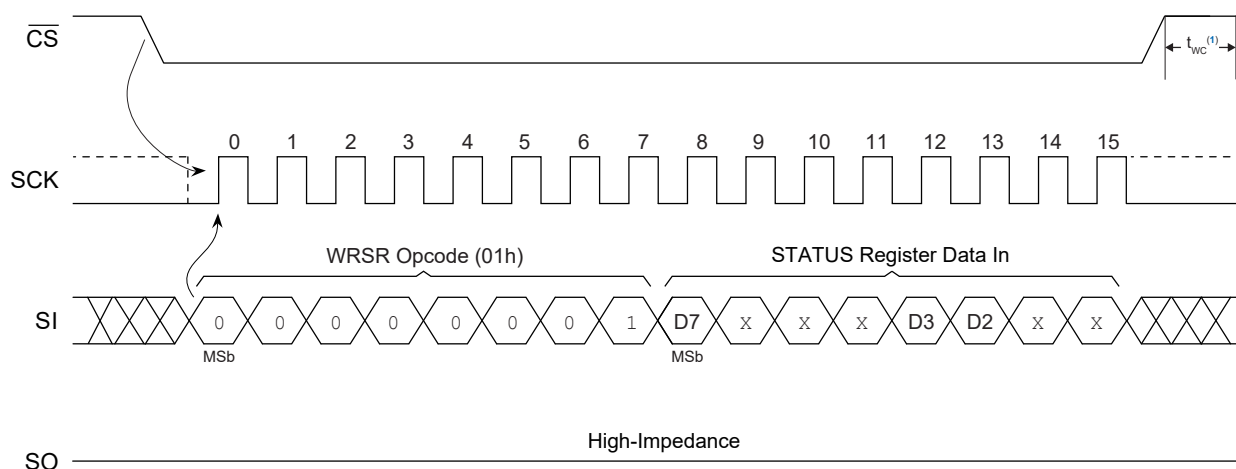
Figure 6-4. WRSR Waveform
