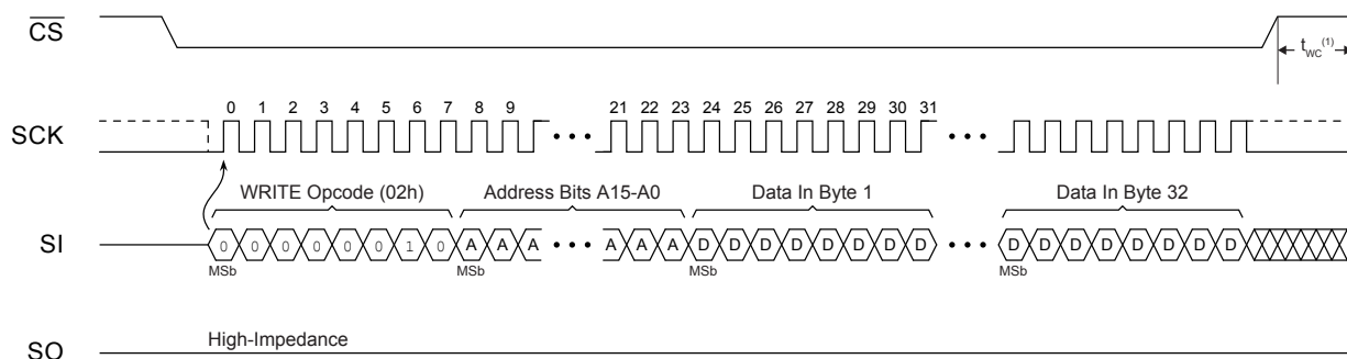
Figure 8-2. Page Write
