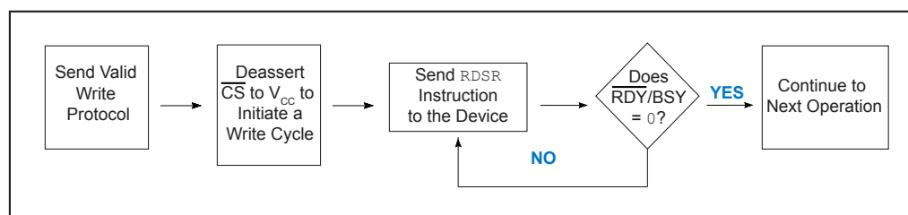
Figure 8-3. Polling Flowchart
