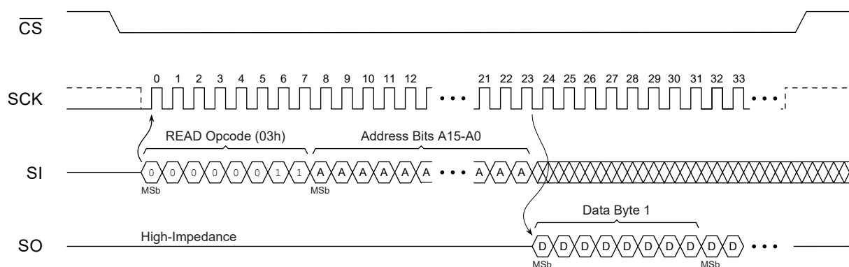
Figure 7-1. Read Waveform
