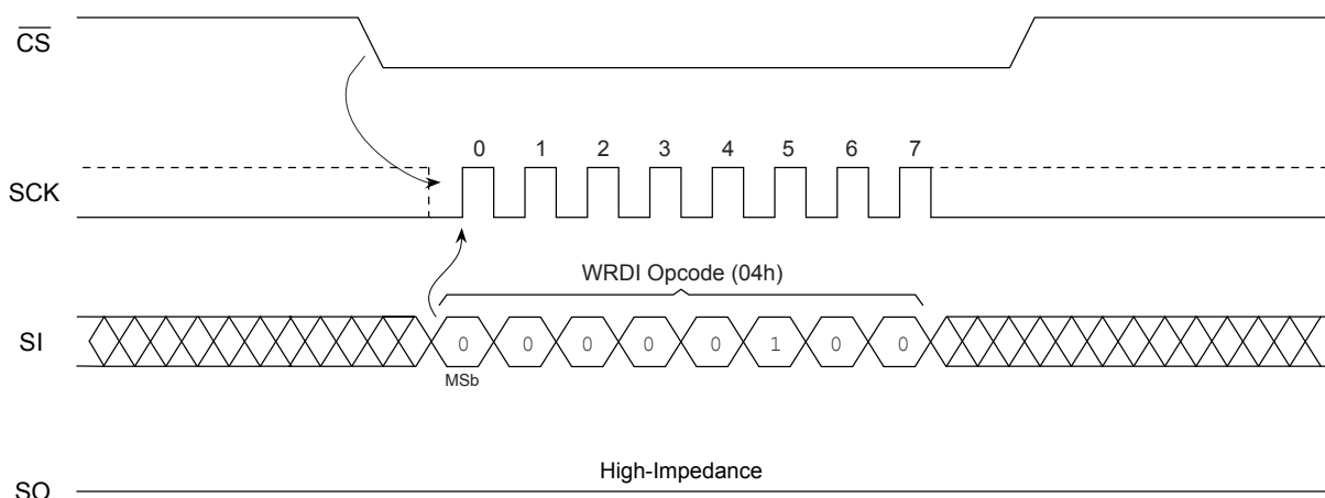
Figure 6-3. WRDI Timing
