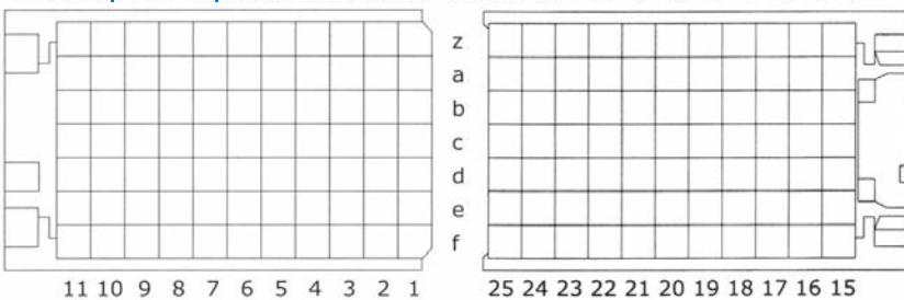
Type-M Connector
