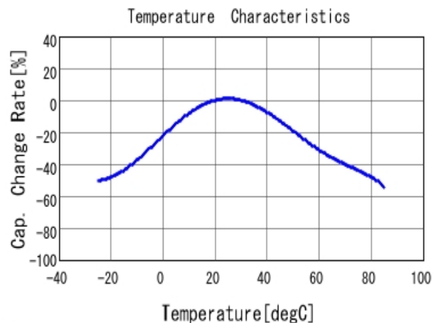
■ DE1E3RB222MA4BR01F C-Temp. capchange, DC0V, AC1Vrms
