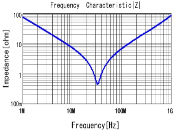
■ DE1E3RB222MA4BR01F |Z| DC0V, 20degC
