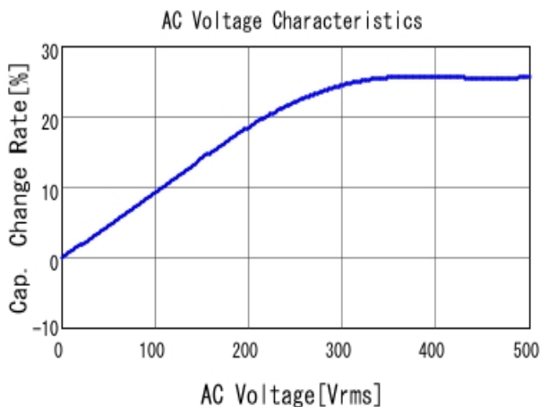
■ DE1E3RB222MA4BR01F C-AC Voltage capchange, DC0V, 20.0
