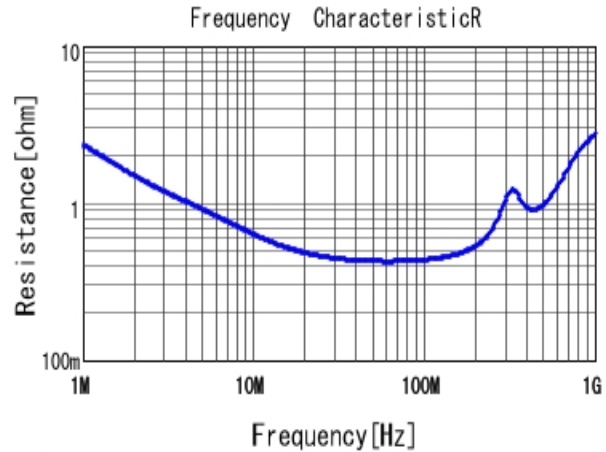
■ DE1E3RB222MA4BR01F R DC0V, 20degC
