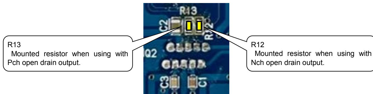
Figure 3 R12,R13 land
