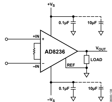
Figure 37. Supply Decoupling, REF, and Output Referred to Ground
