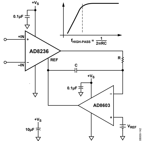
Figure 41. AC-Coupled Circuit
