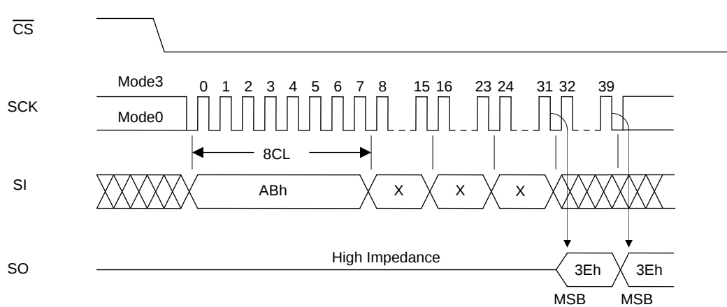
Figure 15-b ID Read
