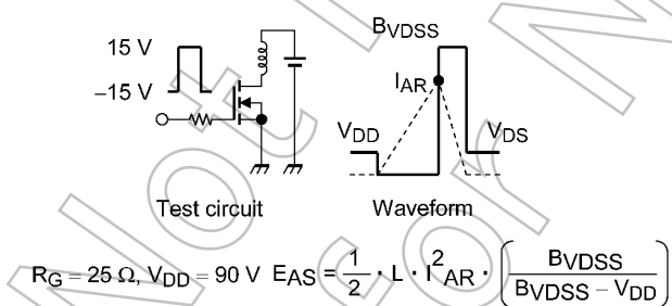
Fig. 8.16 Test Circuit/Waveform
