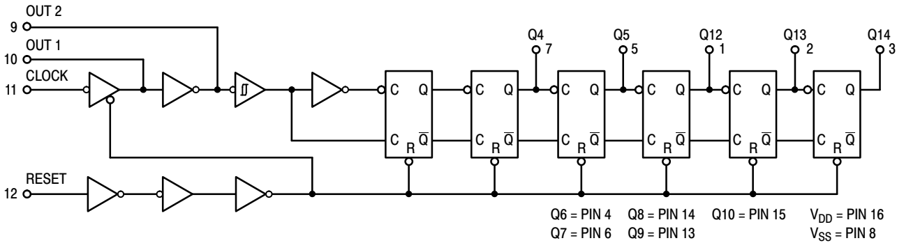
Figure 1. Logic Diagram
