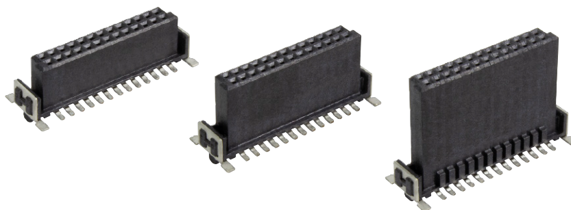
Female connectors, straight, SMT
