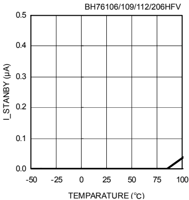
Fig.16 Temperature-Standby Circuit Current
