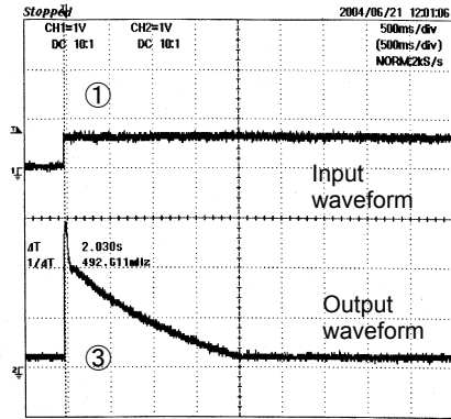
Fig10 Relationship of Output Voltage to Input Voltage (For BH76106HFV C_{in}=1\mu\text{F} )
