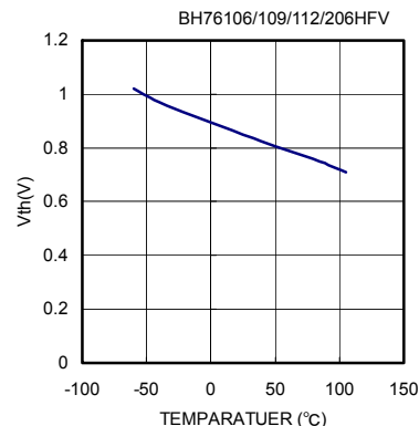
Fig.28 Temperature-V th
