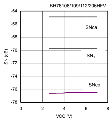
Fig.25 Supply Voltage-S/N
