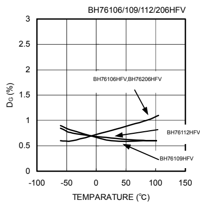
Fig.22 Temperature-D G
