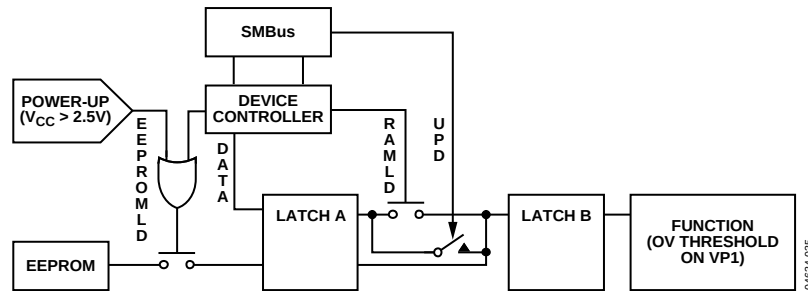
Figure 25. Configuration Update Flow Diagram
