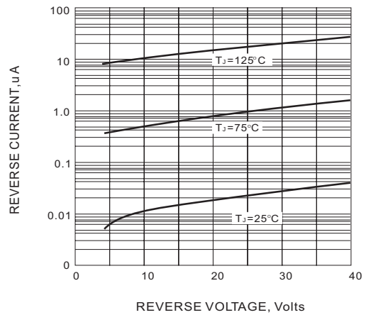
FIG. 2-TYPICAL REVERSE CHARACTERISTICS
