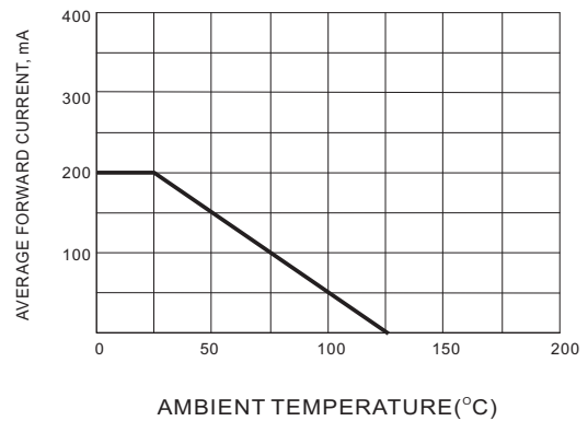
FIG. 4 FORWARD CURRENT DERATING
