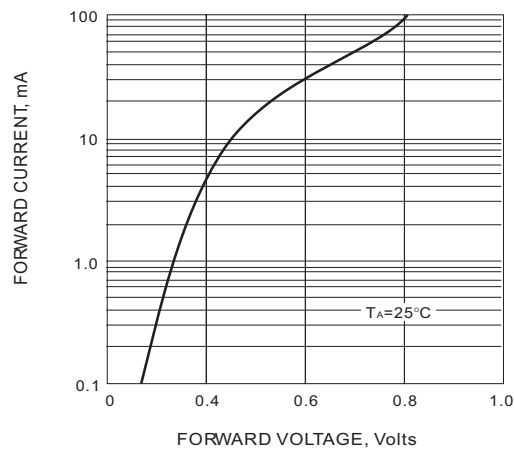
FIG. 1-TYPICAL FORWARD CHARACTERISTIC
