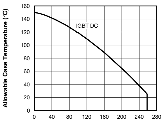
Fig. 1 - Maximum DC IGBT Collector Current vs. Case Temperature
