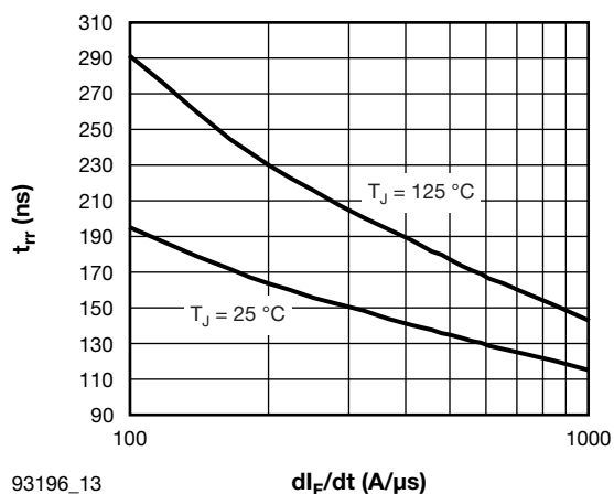
Fig. 13 - Typical t_{rr} Diode vs. dI_F/dt V_{rr} = 400\text{ V} , I_F = 50\text{ A}
