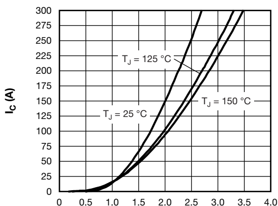
Fig. 3 - Typical IGBT Collector Current Characteristics V_{GE} = 15 V
