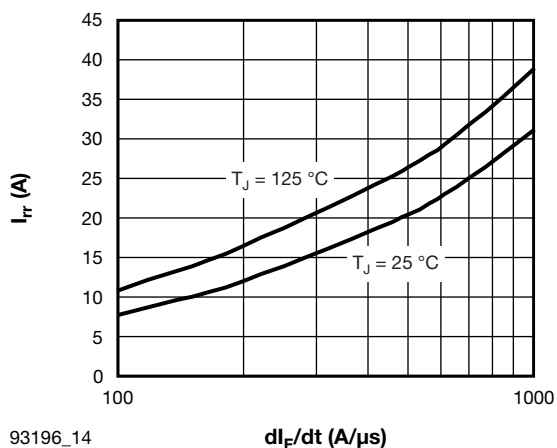
Fig. 14 - Typical I_{rr} Diode vs. dI_F/dt V_{rr} = 400\text{ V} , I_F = 50\text{ A}
