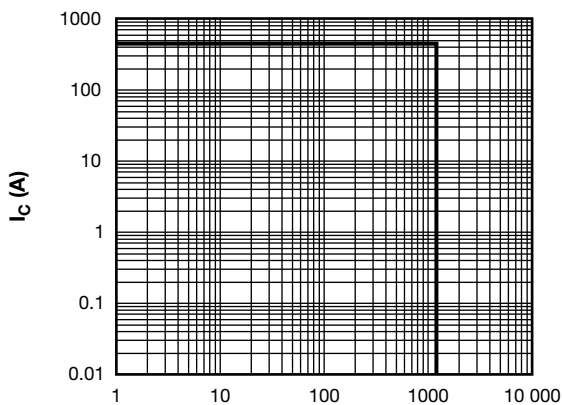
Fig. 2 - IGBT Reverse Bias SOA T_J = 150 °C, V_{GE} = 15 V
