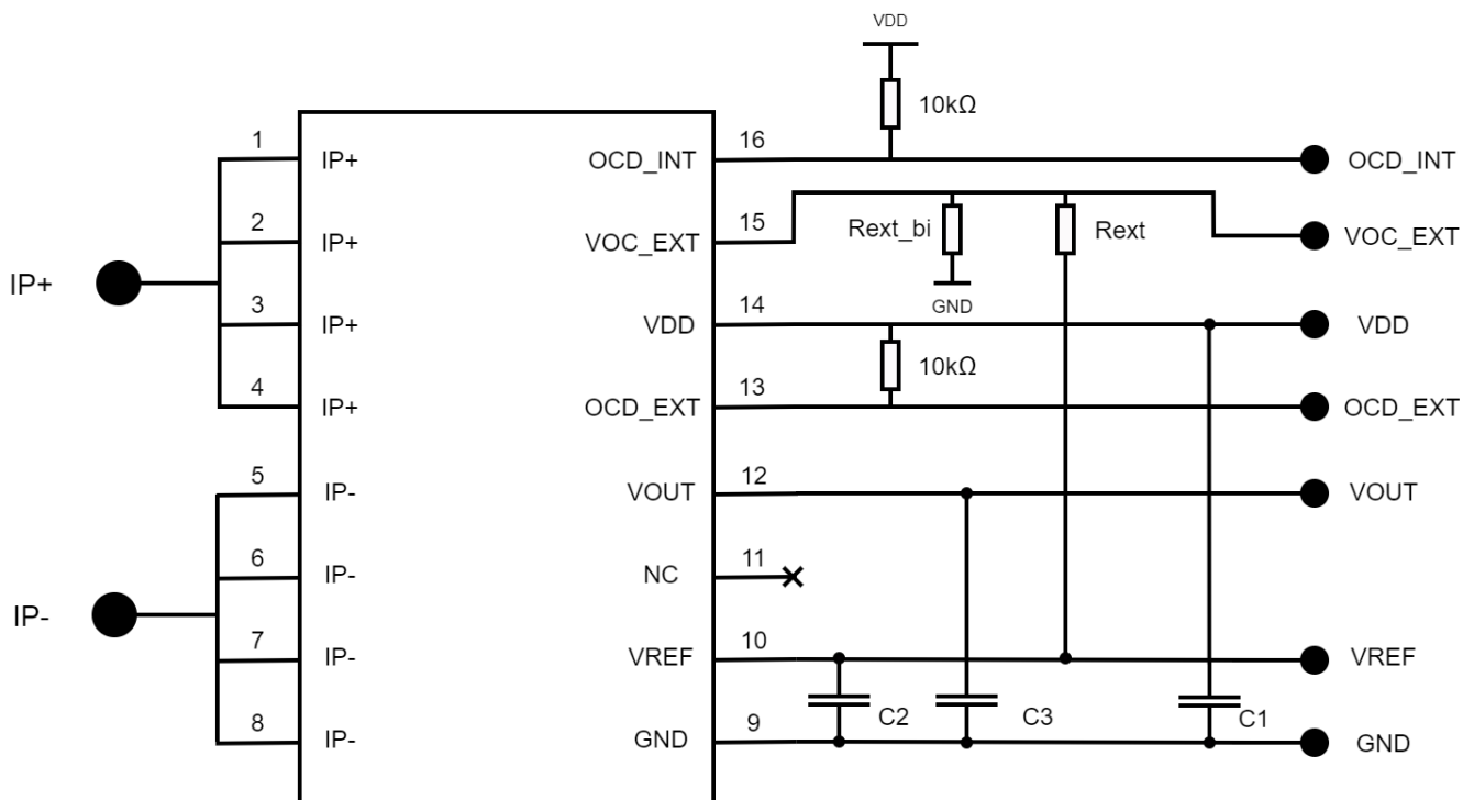
Figure 7: Recommended wiring for the MLX91221 with Bidirectionnal OCD_{EXT}
