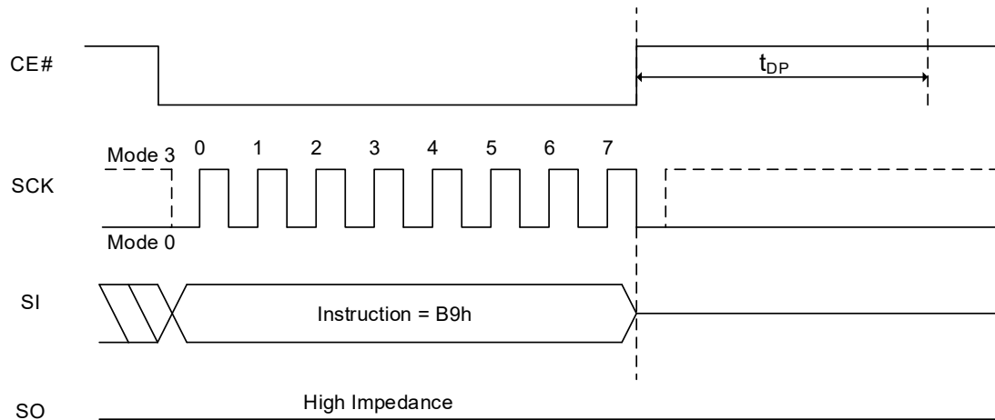
Figure 8.33 Enter Deep Power Down Mode Sequence
