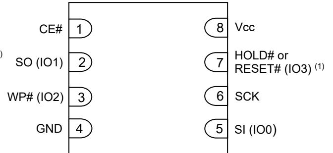
8-contact WSON 6x5mm 8-contact WSON 8x6mm 8-contact XSON 4x4mm
