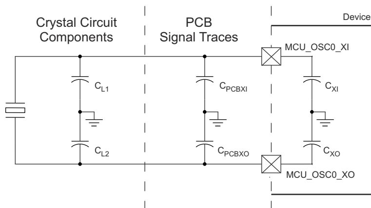
Figure 7-18. Load Capacitance
