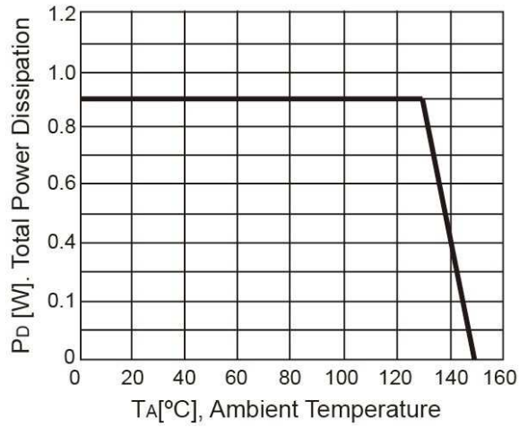
Figure 7. Power Dissipation vs. Ambient Temperature
