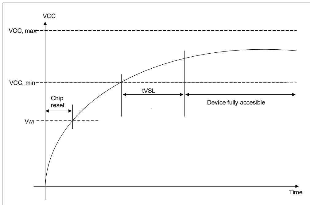
Figure 8.26 Power-Up Timing
