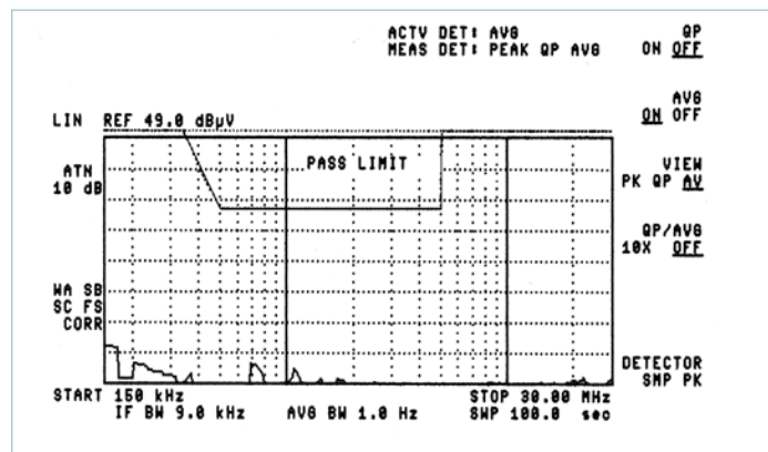
Figure 9.10c — Average detection
