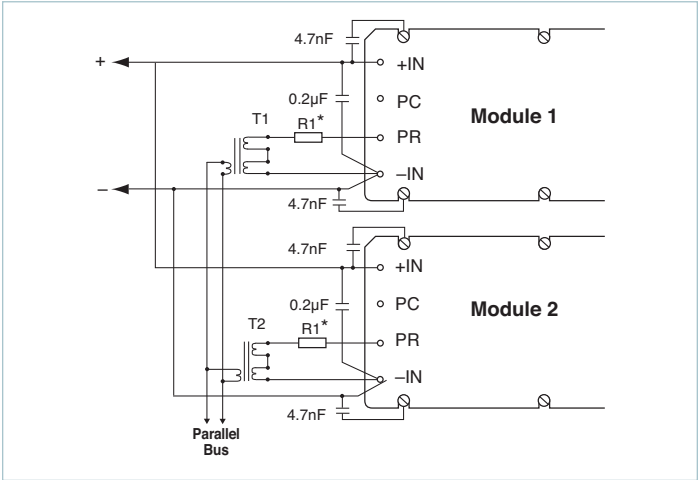
Figure 2.8 — Transformer-coupled interface
