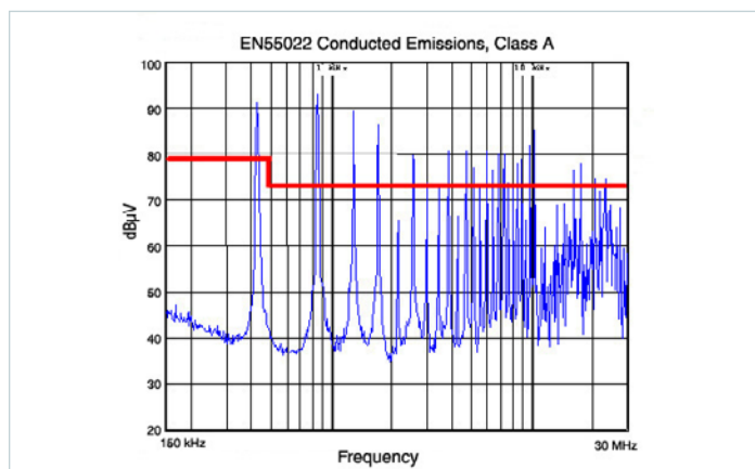
Figure 4.2 — V48B28H250BN without bypass caps (330μF across input)
