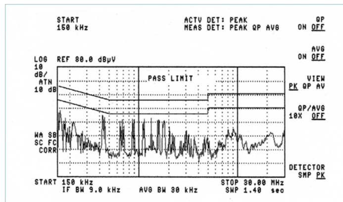
Figure 9.10a — Peak detection
