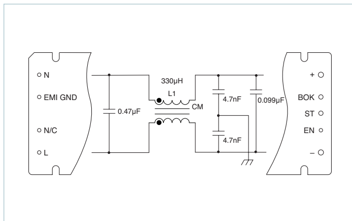
Figure 8.6 — Internal filter
