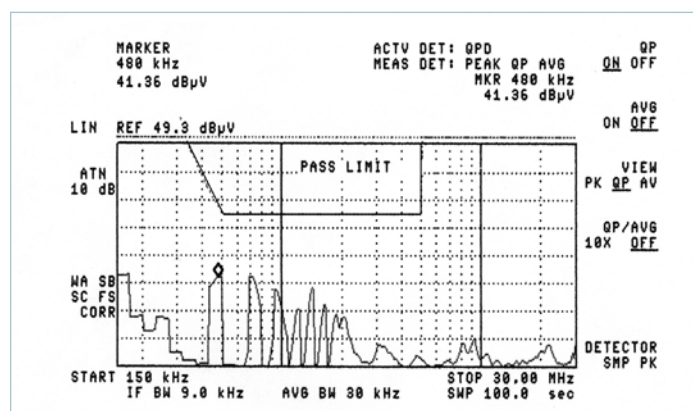
Figure 9.10b — Quasi-peak detection
