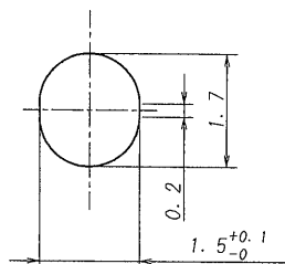
DETAIL. J
