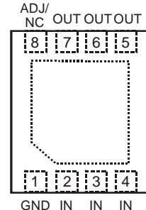
U-DFN2030-8
