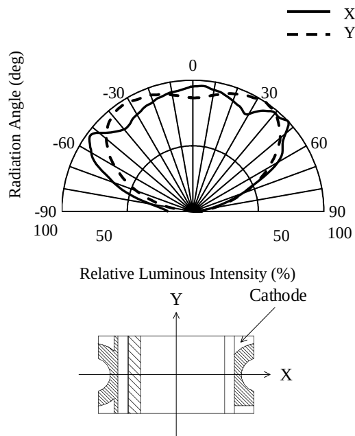
Figure 6. Directivity
