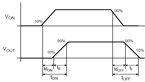
Figure 27. Timing Diagram
