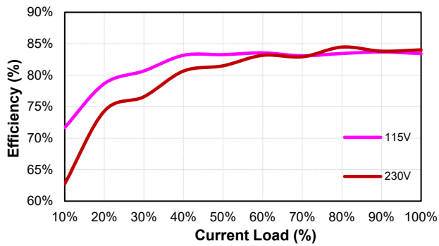
CFM60S090 (Eff Vs Io)
