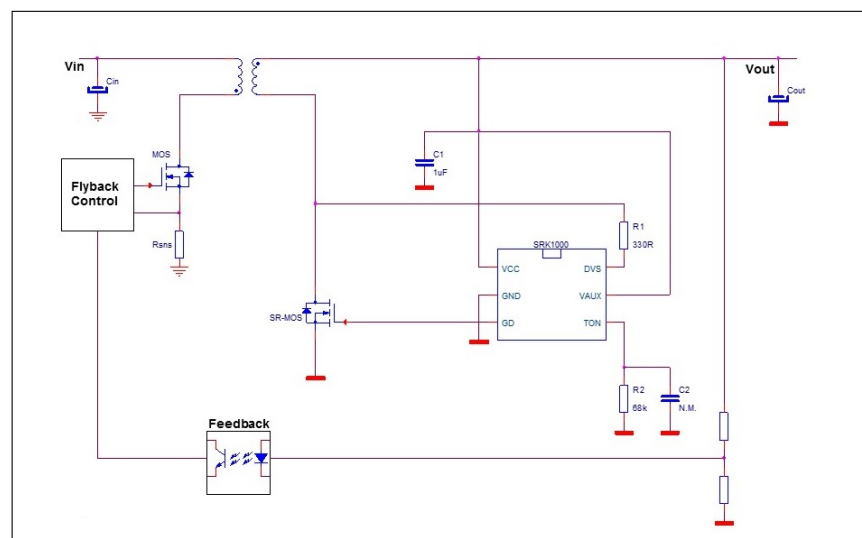
Figure 4. QR flyback adapter (CV regulation)
