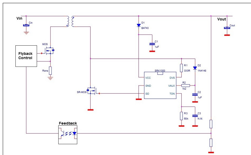
Figure 3. QR flyback charger with CV-CC regulation
