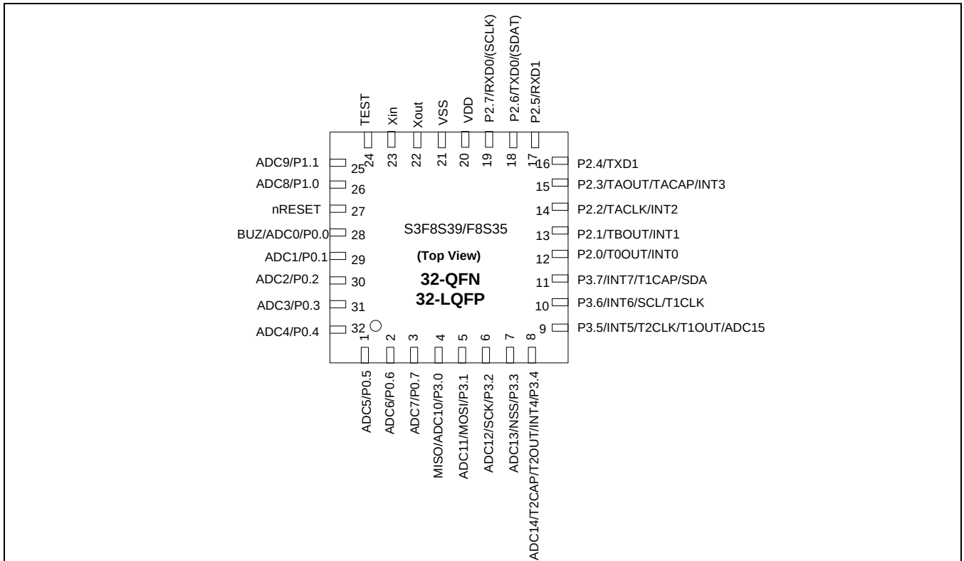
Figure 1-3 S3F8S39/S3F8S35 Pin Assignment (32-QFN/32-LQFP)
