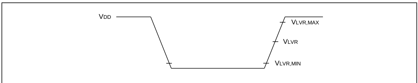
Figure 23-6 LVR Reset Timing
