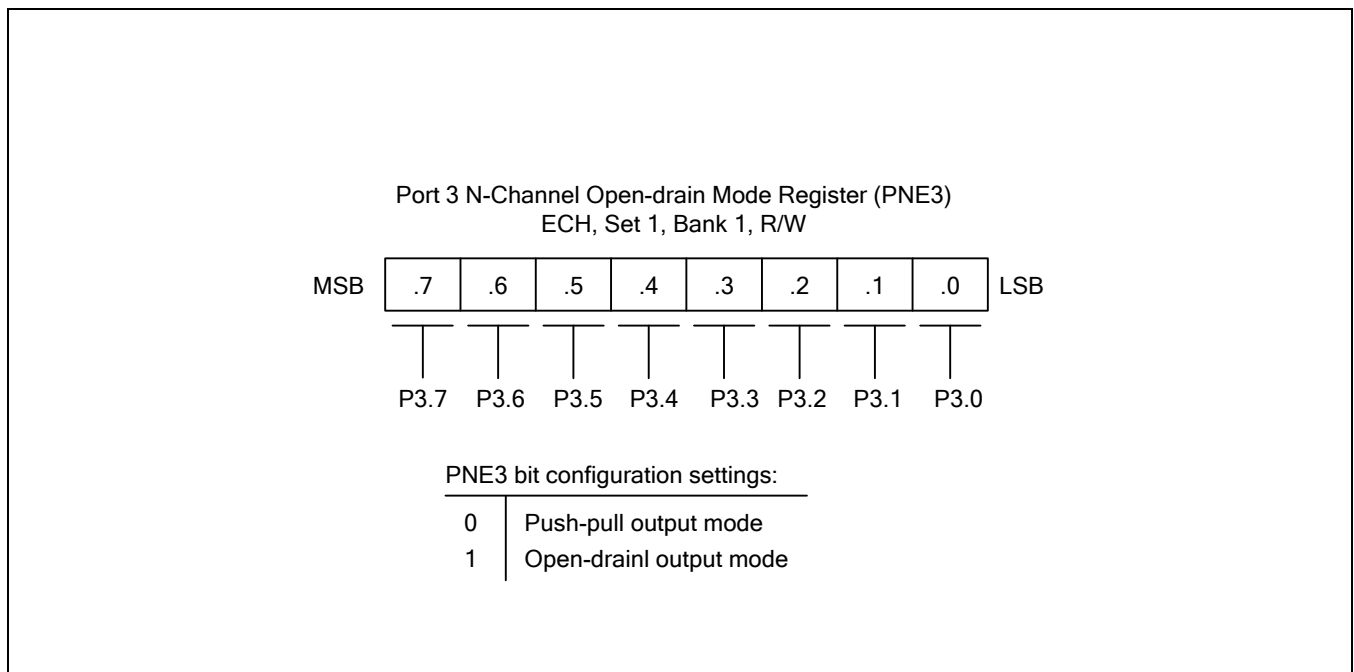
Figure 9-14 Port 3 N-Channel Open-Drain Mode Register (PNE3)
