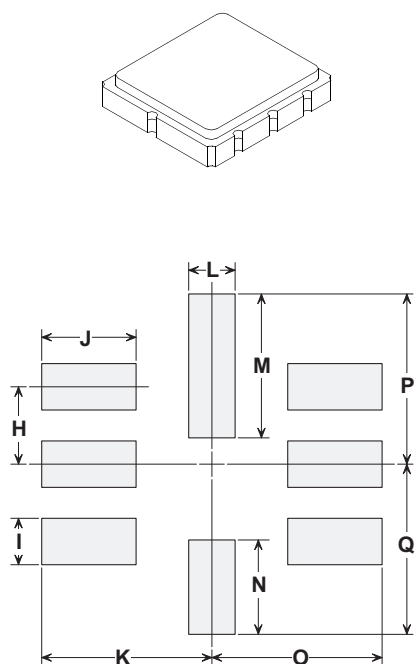
PCB Footprint
