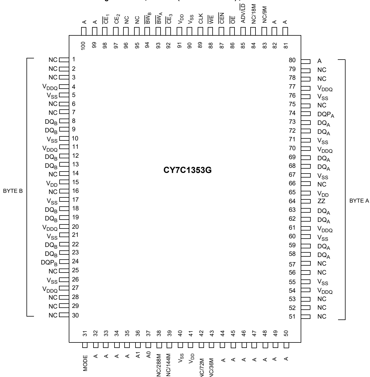
Figure 1. 100-pin TQFP (14 × 20 × 1.4 mm) pinout [1]
