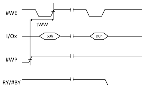
Figure 9-23 Erase Enable
