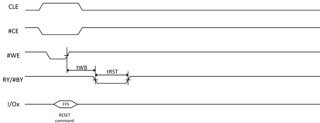
Figure 11-19 Reset
