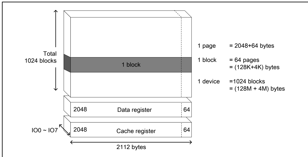
Figure 6-1 Array Organization
