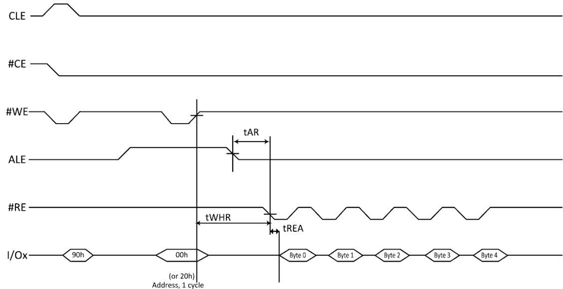
Figure 9-6 Read ID
