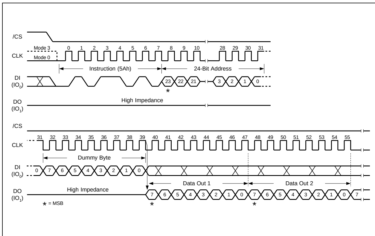
Figure 44. Read SFDP Register Instruction Sequence Diagram(SPI Mode)
