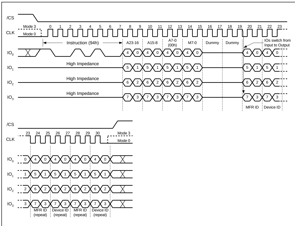
Figure 41a. Read Manufacturer / Device ID Quad I/O Instruction (SPI Mode only)
