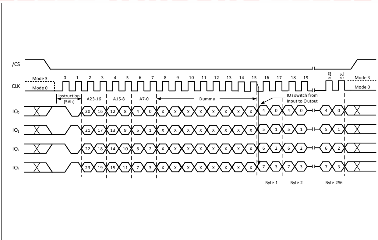
Figure 44. Read QPI Register Instruction Sequence Diagram (QPI Mode)
