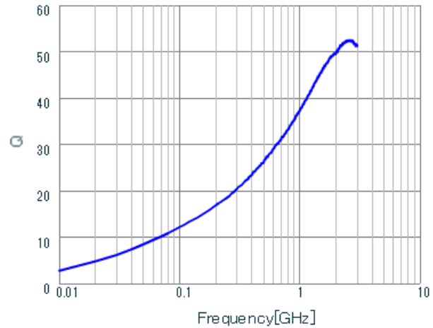
LQG15HN3N9C02 Q.
