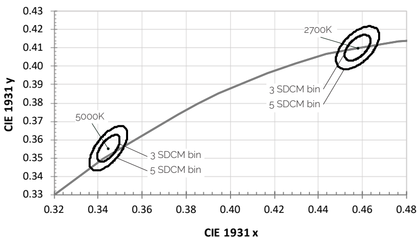
Figure 13: Graph of CCT bins in CIE 1931 Color Space, T_c=85^{\circ}\text{C}
