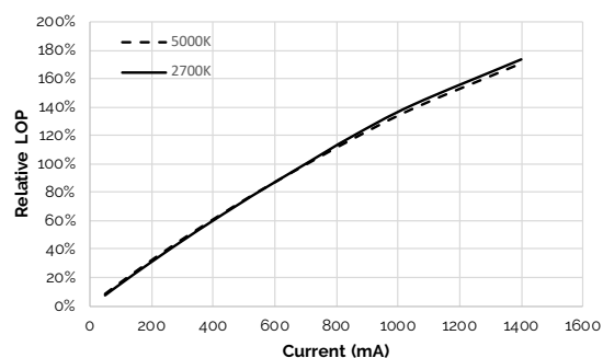
Figure 2: Relative Flux vs. Drive Current, T_c = 25^\circ\text{C}
