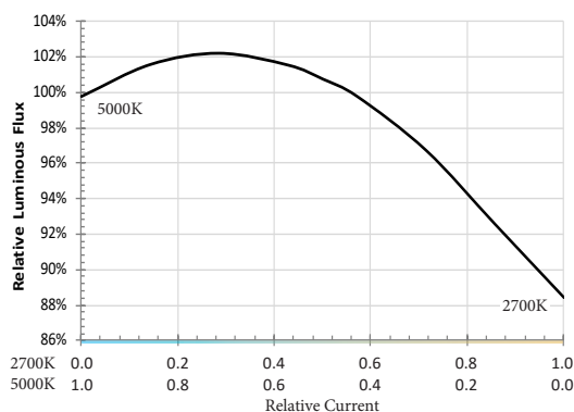
Figure 8: Derating Curve
