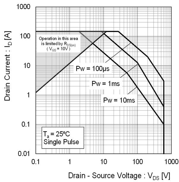
Fig.4 Maximum Safe Operating Area
