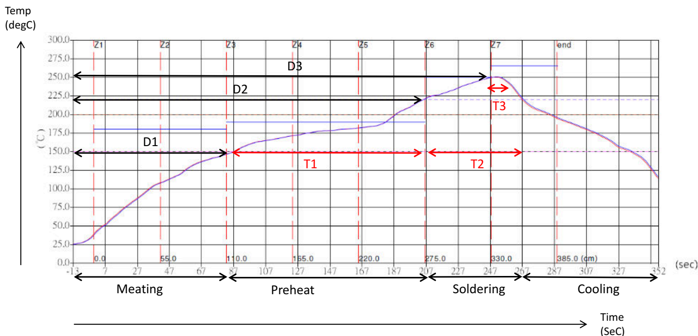
Figure 10-7. Reflow Profile for the WiLink 8 Module
