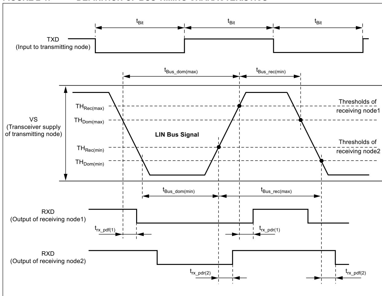
FIGURE 2-1: DEFINITION OF BUS TIMING CHARACTERISTICS
