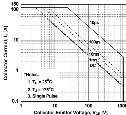
Figure 10. SOA Characteristics
