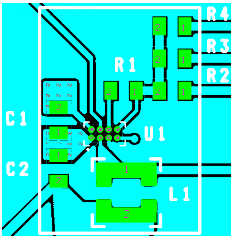
Figure 4. NCP1523B Layout
