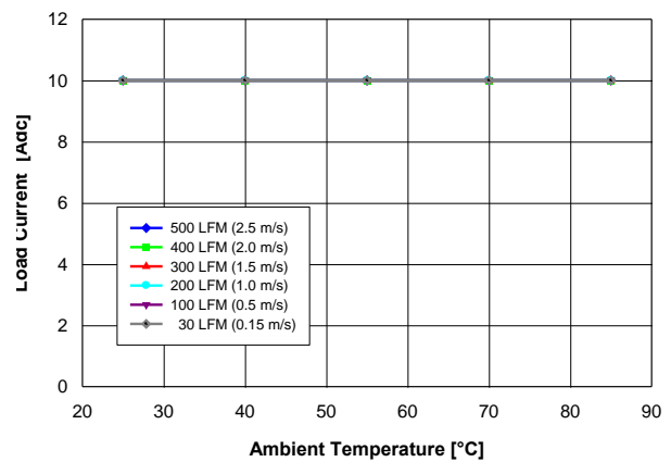
Fig. 2.5V.2: Available load current vs. ambient temperature and airflow rates for V_{out} = 2.5V converter mounted horizontally with air flowing from pin 10 to pin 1, and maximum MOSFET temperature \leq 120^\circ C .
