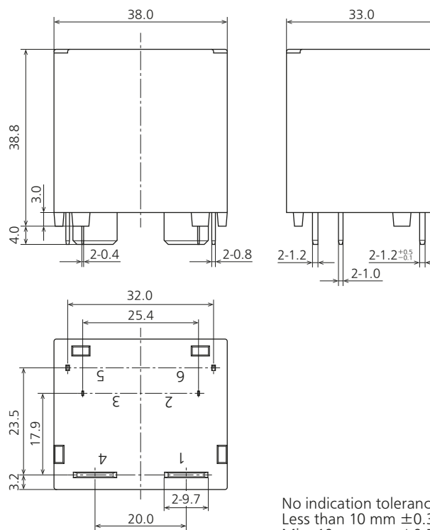
External dimensions
