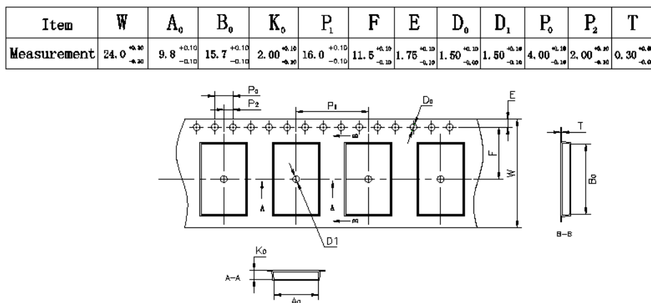
Figure 10. CYBLE-224116-01 Tape Dimensions
