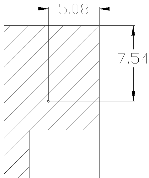
Figure 13. CYBLE-224116-01 Center of Mass (Seen from Top)
