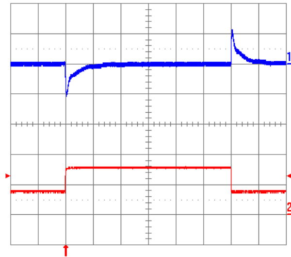
Fig. 2.5V.12: Output voltage response to load current step-change (3.75 A – 7.5 A – 3.75 A) at V_{in} = 48V . Top trace: output voltage (100 mV/div.). Bottom trace: load current (5A/div.). Current slew rate: 5 A/ \mu s . C_o = 450\mu F tantalum + 1 \mu F ceramic. Time scale: 0.2 ms/div.
