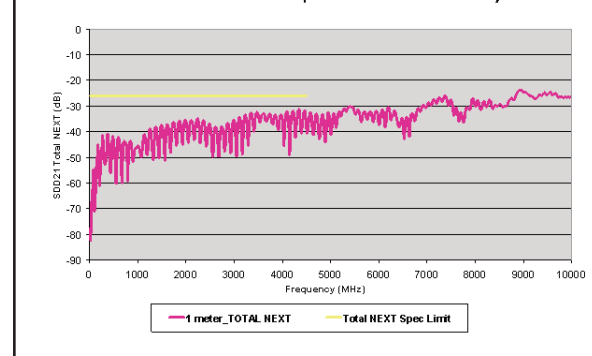
Total NEXT of 4x Mini-SAS unequalized 1 meter cable assembly
