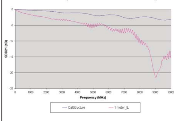
Insertion Loss of unequalized 1 meter 4X Mini-SAS Cable Assembly
