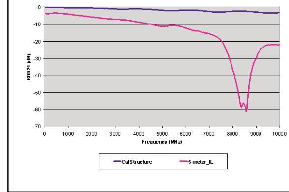
Insertion Loss of equalized 5 meter 4X Mini-SAS Cable Assembly
