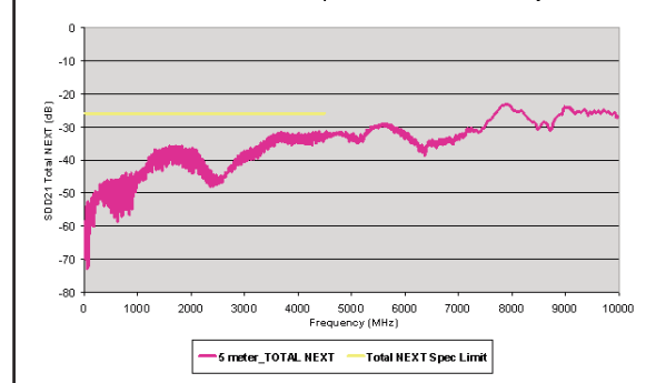
Total NEXT of 4x Mini-SAS equalized 5 meter cable assembly
