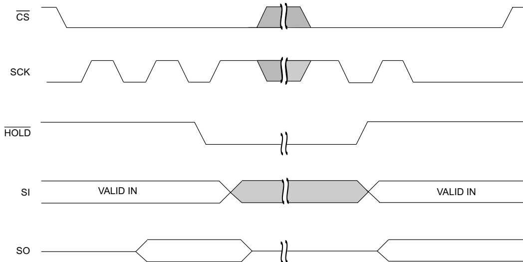
Figure 13. HOLD Operation [2]
