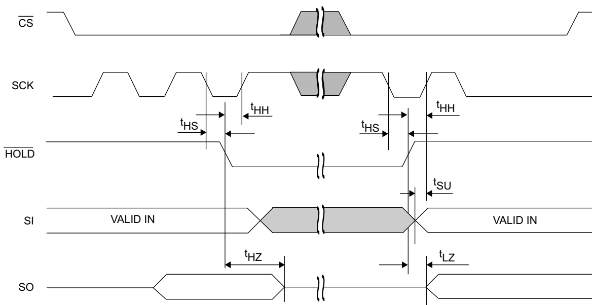
Figure 15. HOLD Timing
