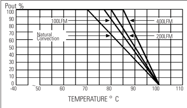
MODEL 100HFS Single - 3.3V, 5V & ±5V Output
