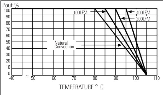
MODEL 100HFS Dual - all other outputs
