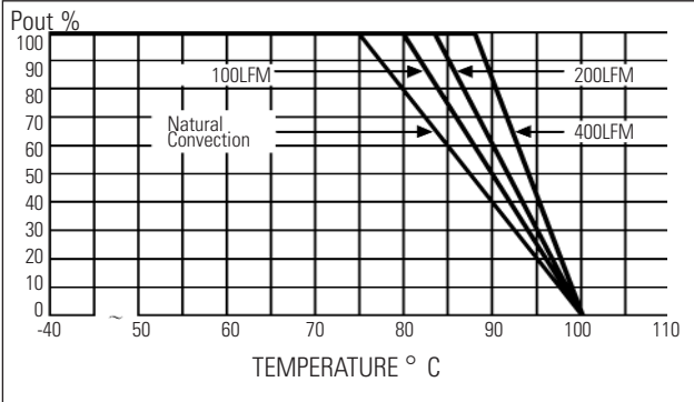
MODEL 100HFS Single - 24V
