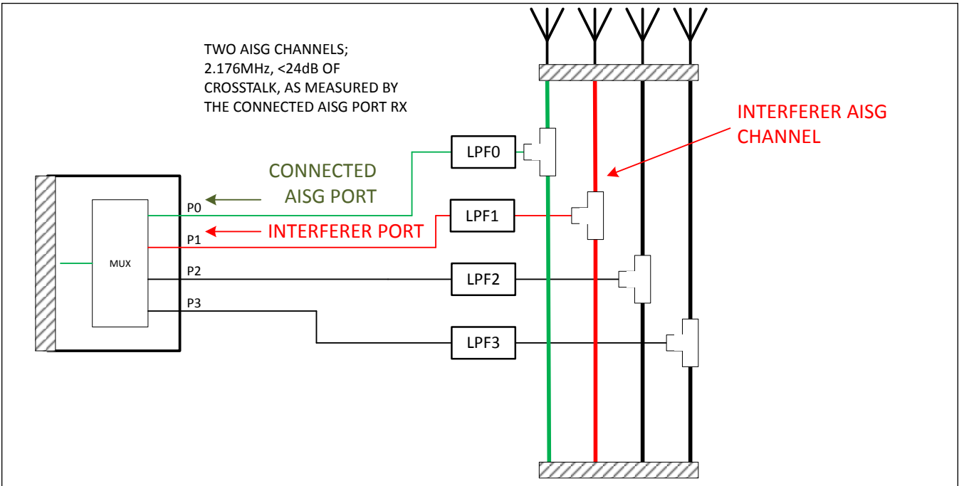
Figure 6. Modem Crosstalk
