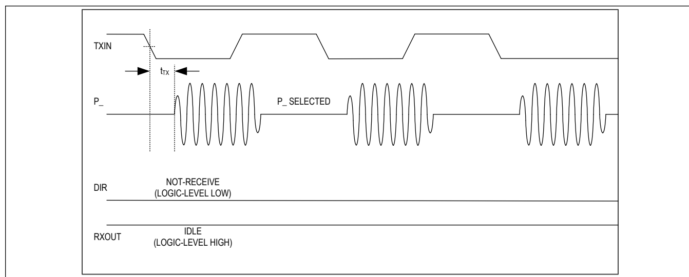
Figure 8. Transmitter Timing
