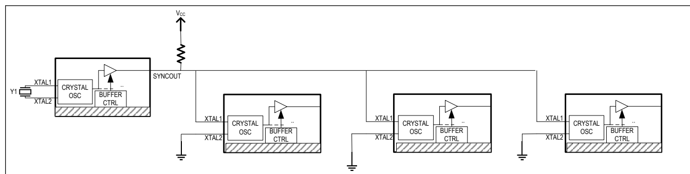
Figure 26. Star Daisy-Chain
