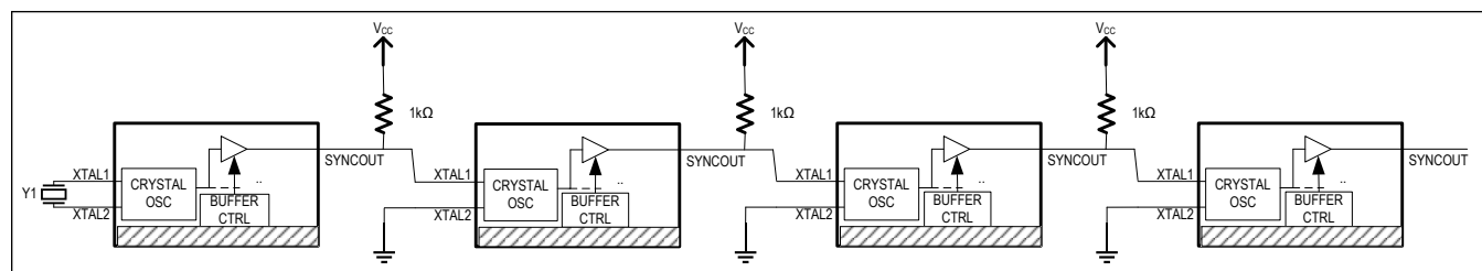
Figure 25. Cascade Daisy-Chain
