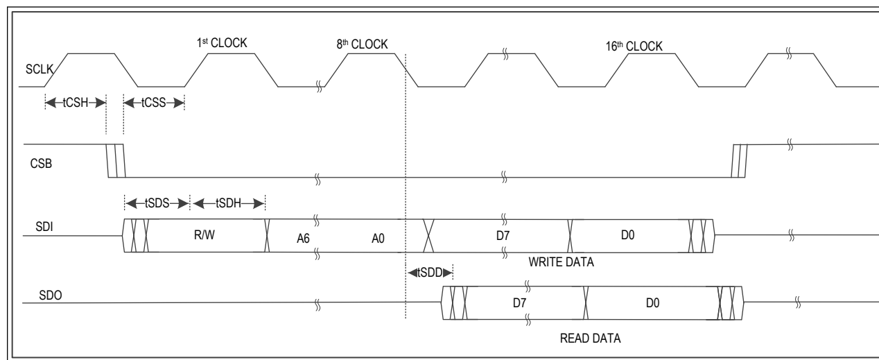
Figure 1. SPI Timing
