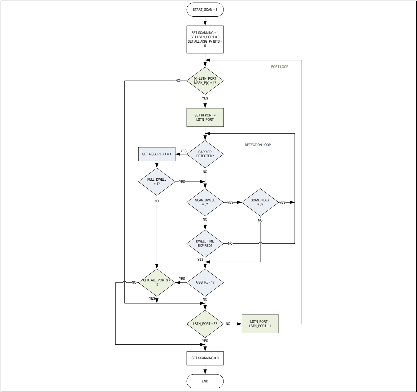
Figure 14. Port Scan Flow Chart
