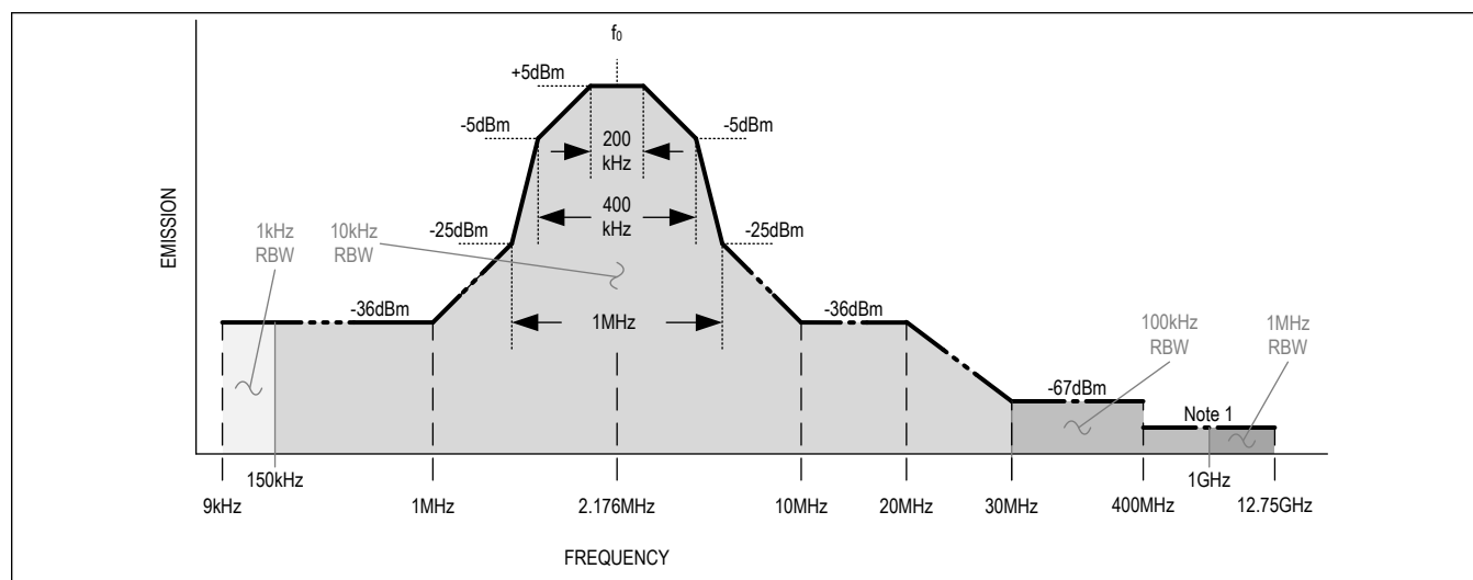
Figure 15. AISG v3.0 Standard Modem Spectrum Emissions Mask
