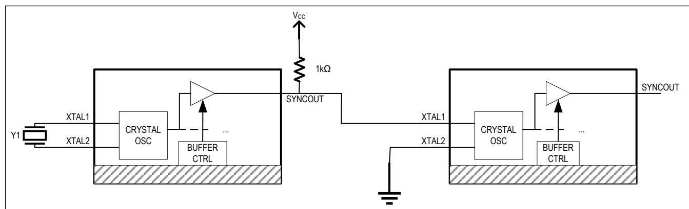
Figure 24. Clock Transmitter/Receiver Circuit
