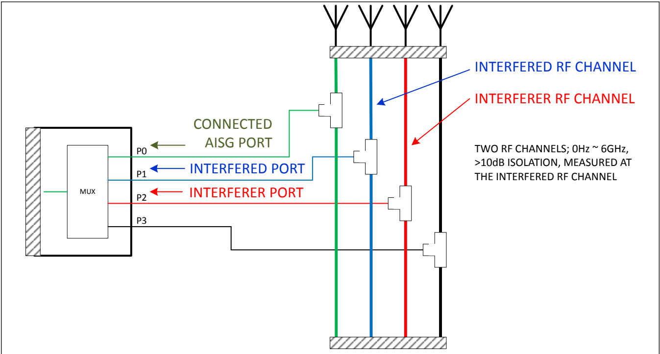
Figure 4. RF Isolation
