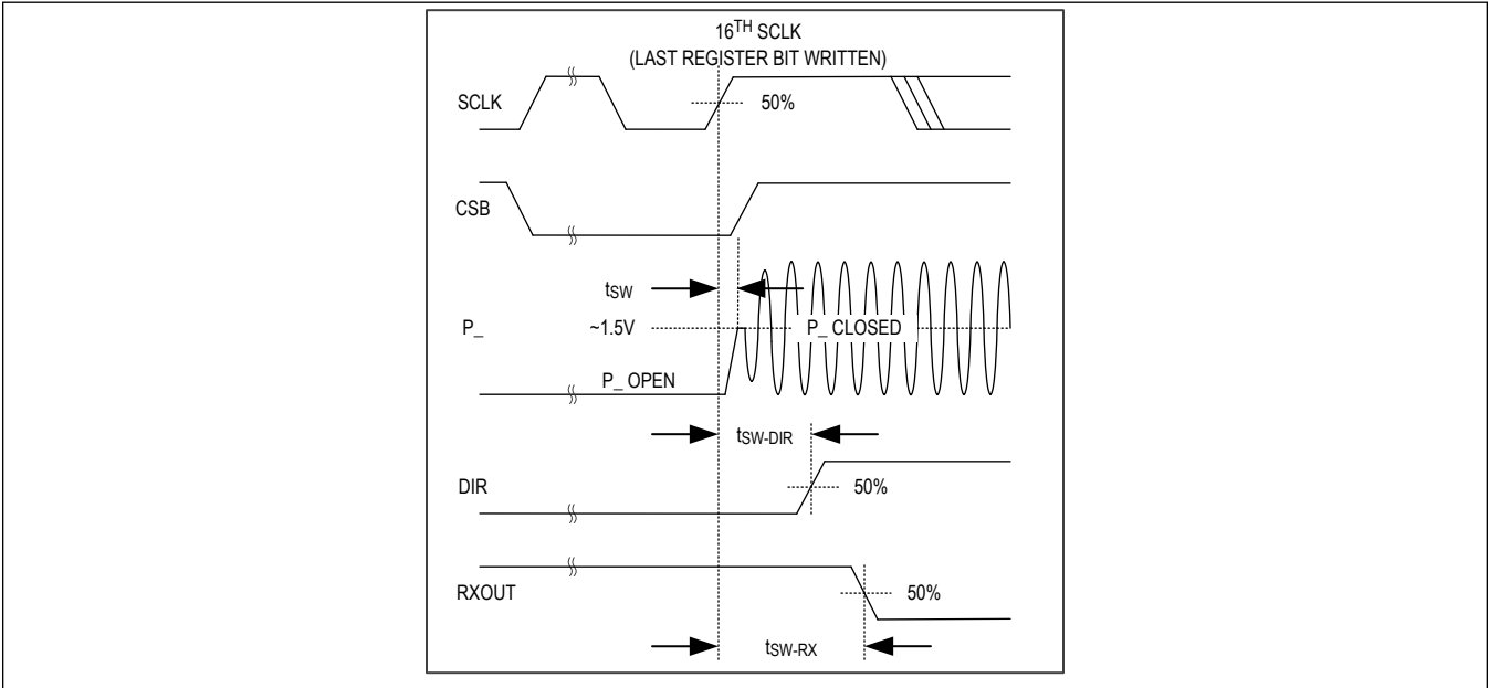
Figure 3. Switch Timing
