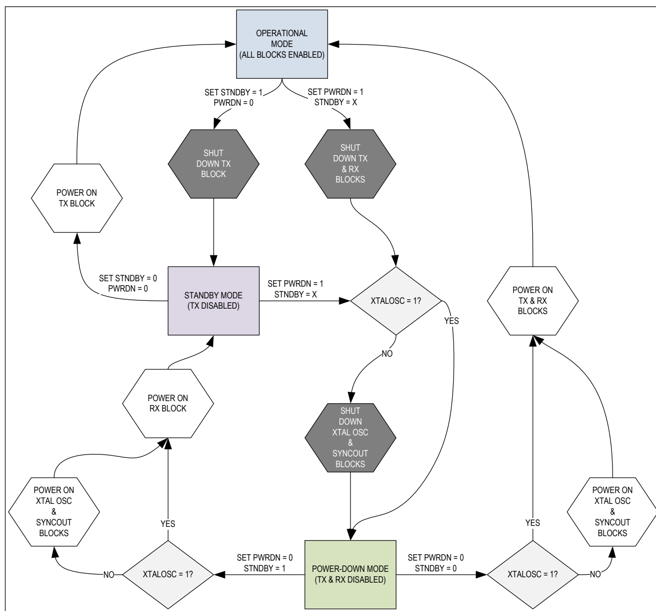
Figure 13. Power Modes
