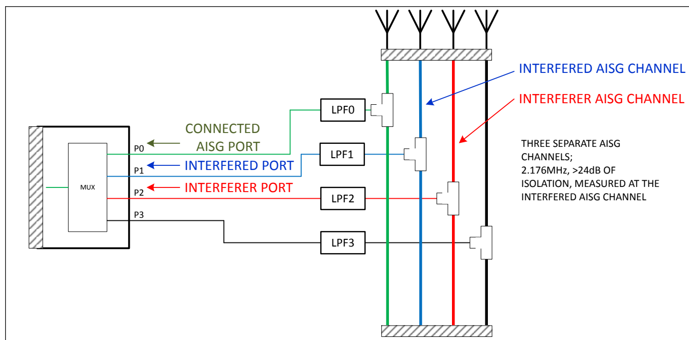
Figure 5. AISG Isolation
