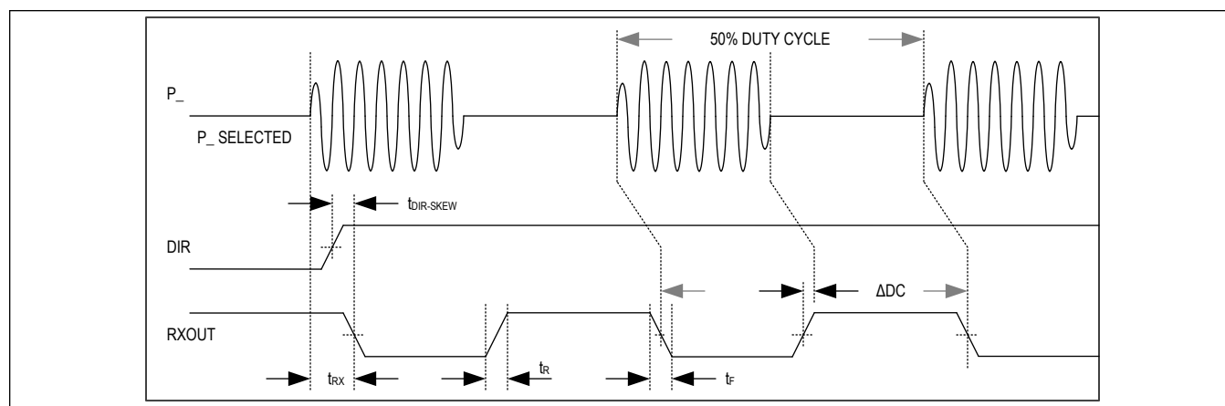
Figure 7. Receiver Timing
