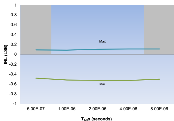
Figure 39-8. ADC 10-bit, INL, V_{DD} = 3.0V , V_{REF} = 3.0V , Min and Max values at 125^{\circ}C + 3\sigma
