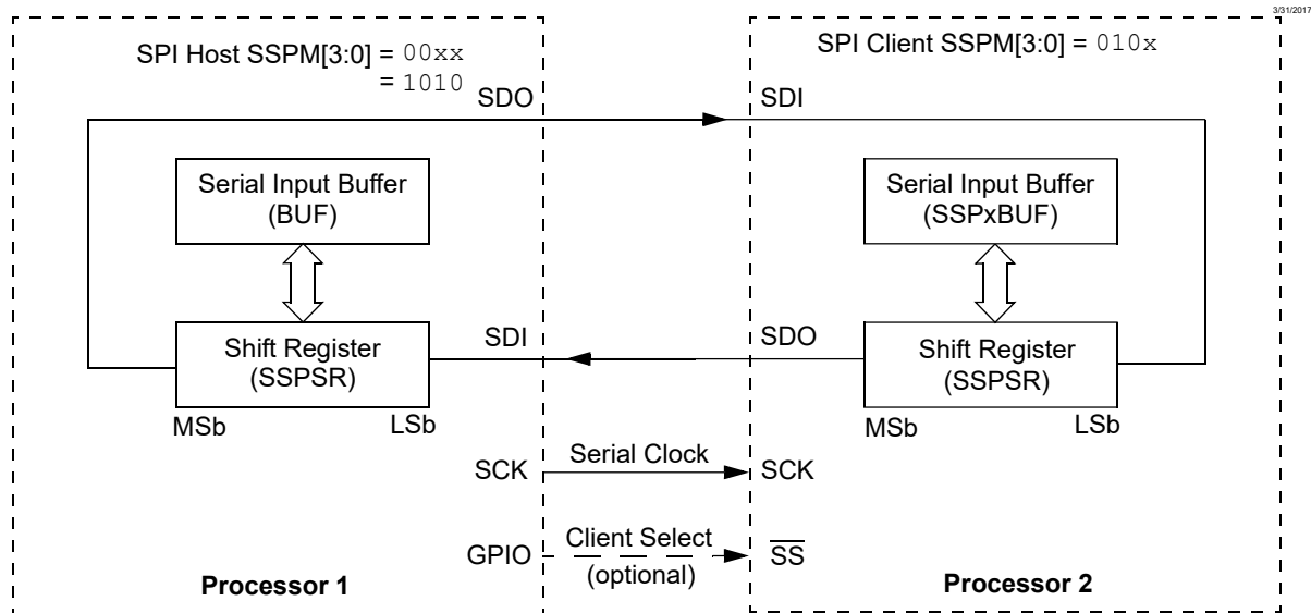
Figure 27-3. SPI Host/Client Connection
