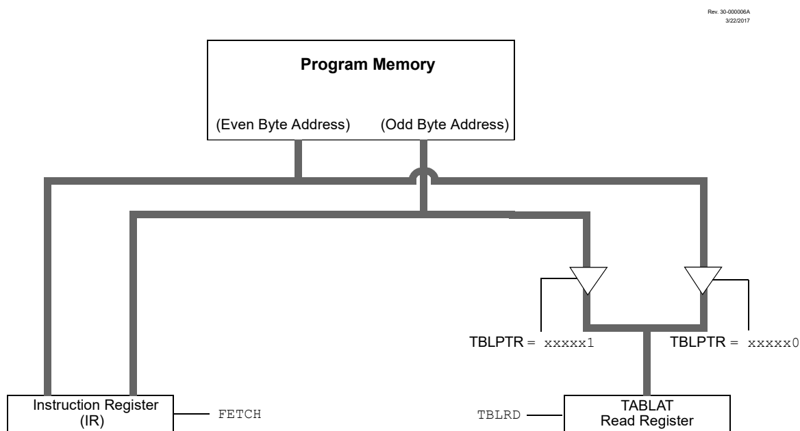
Figure 12-5. Program Flash Memory Read Flowchart
