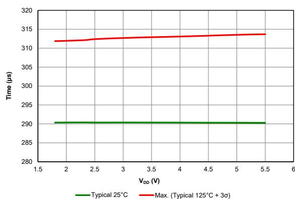
Figure 39-56. Wake from Sleep, VREGPM = 01
