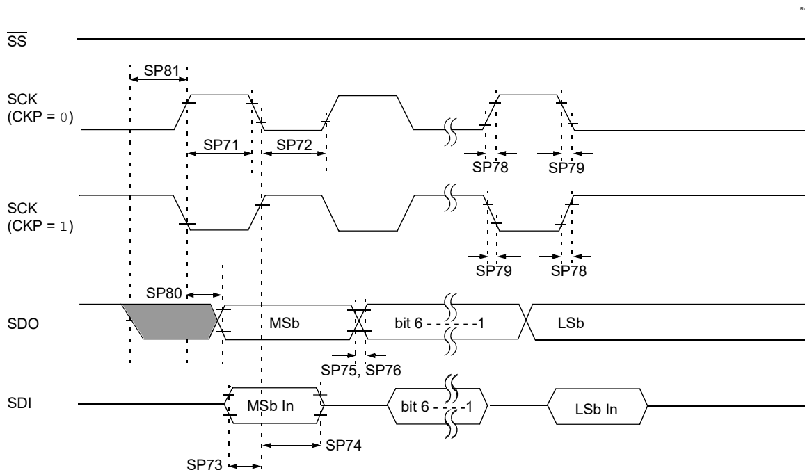
Figure 38-15. SPI Host Mode Timing (CKE = 0, SMP = 0)
