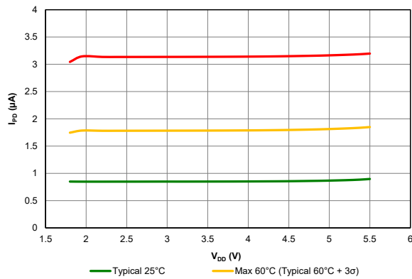
Figure 39-49. I_{PD} Base (VREGPM = 10)
