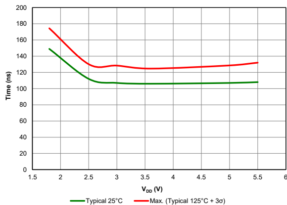
Figure 39-27. Comparator Response Time Falling edge
