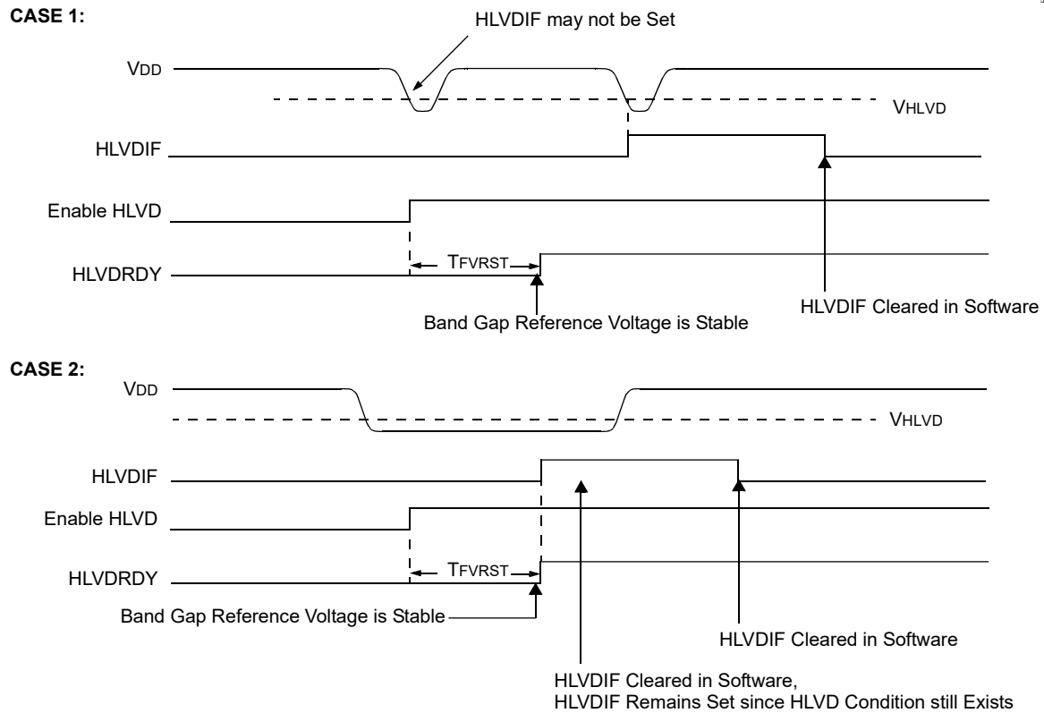
Figure 34-2. Low-Voltage Detect Operation (INTL = 1)
