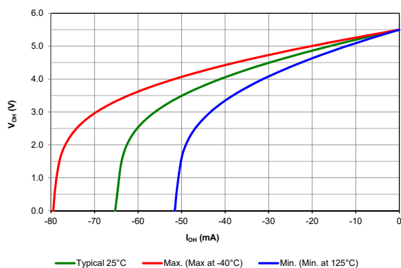
Figure 39-76. V_{OH} vs. I_{OH} over Temperature, V_{DD} = 5.5V
