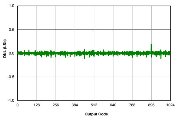
Figure 39-3. ADC, DNL, V_{DD} = 3.0V , T_{AD} = 1 \mu s , 25^\circ C
