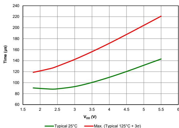
Figure 39-55. Wake from Sleep, VREGPM = 10, HFINTOSC = 16 MHz
