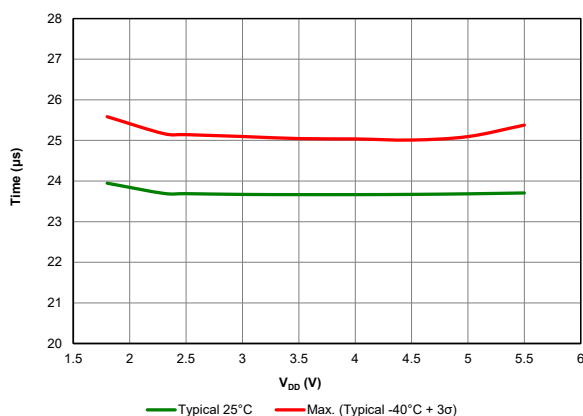
Figure 39-54. Wake from Sleep, VREGPM = 0x, HFINTOSC = 16 MHz
