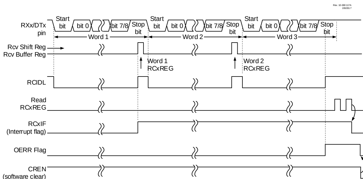
Figure 28-5. Asynchronous Reception
