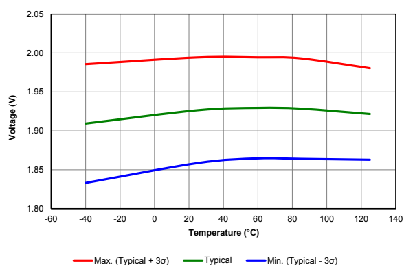
Figure 39-58. Low-Power Brown-Out Reset Rearm Voltage
