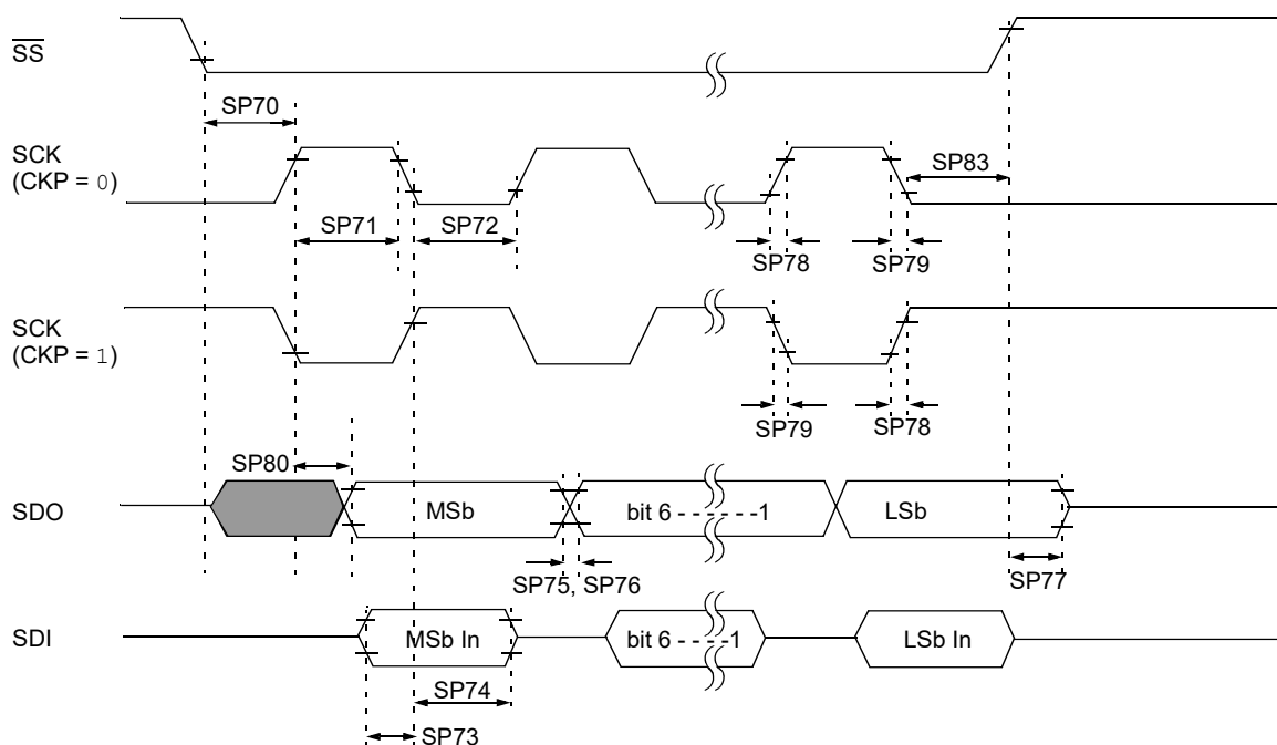
Figure 38-17. SPI Client Mode Timing (CKE = 0)
