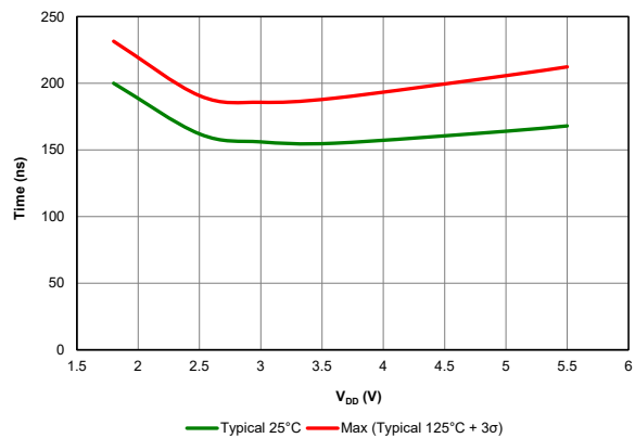
Figure 39-28. Comparator Response Time Rising edge
