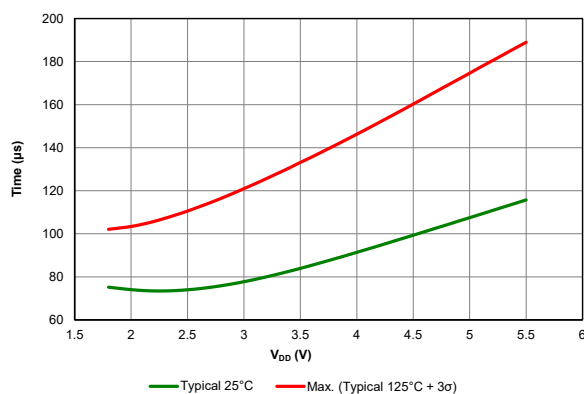
Figure 39-53. Wake from Sleep, VREGPM = 10, HFINTOSC = 4 MHz
