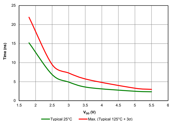
Figure 39-34. Rise Time, Slew Rate Control Disabled
