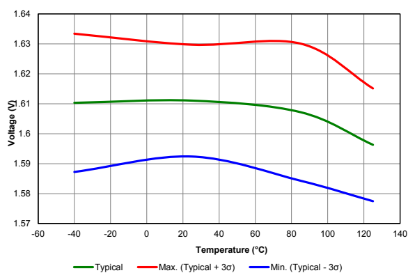
Figure 39-63. POR Release Voltage (VREGPM = 1x)
