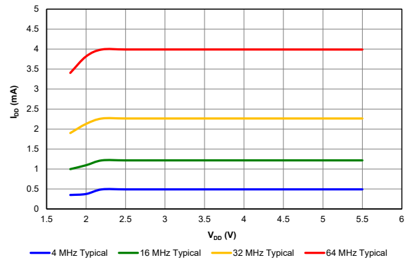
Figure 39-37. I_{DD} , INT Oscillator, Typical
