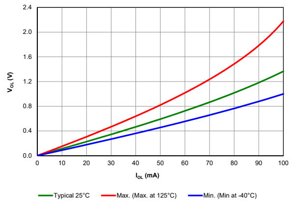
Figure 39-79. V_{OL} vs. I_{OL} over Temperature, V_{DD} = 5.5V
