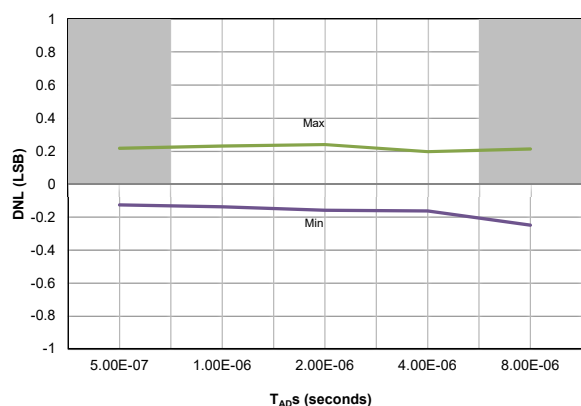
Figure 39-7. ADC 10-bit, DNL, V_{DD} = 3.0V , V_{REF} = 3.0V , Min and Max values at 125^{\circ}C + 3\sigma
