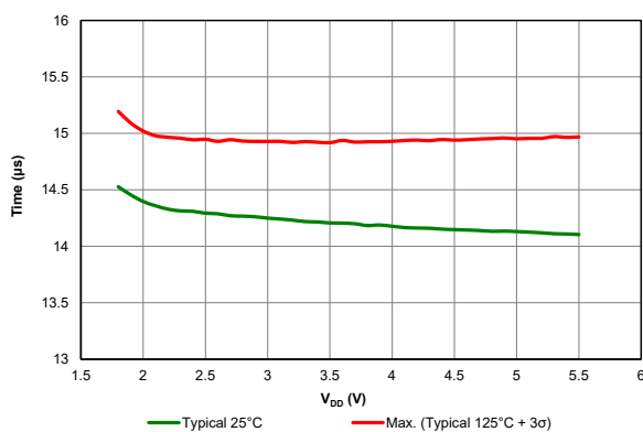
Figure 39-52. Wake from Sleep, VREGPM = 0x, HFINTOSC = 4 MHz
