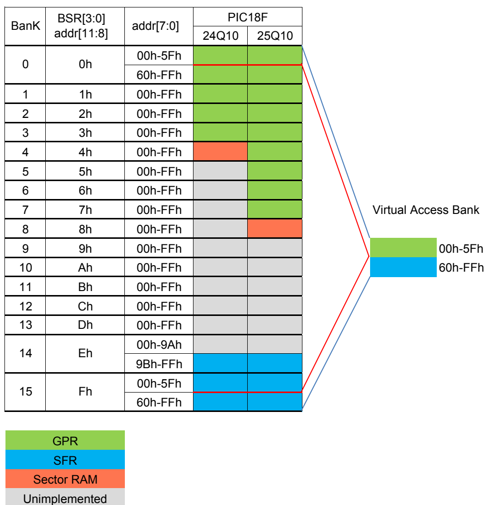
Figure 11-8. Data Memory Map
