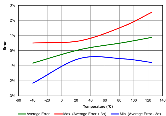
Figure 39-29. FVR Voltage Error 1x ( V_{DD} = 5.5\text{ V} )
