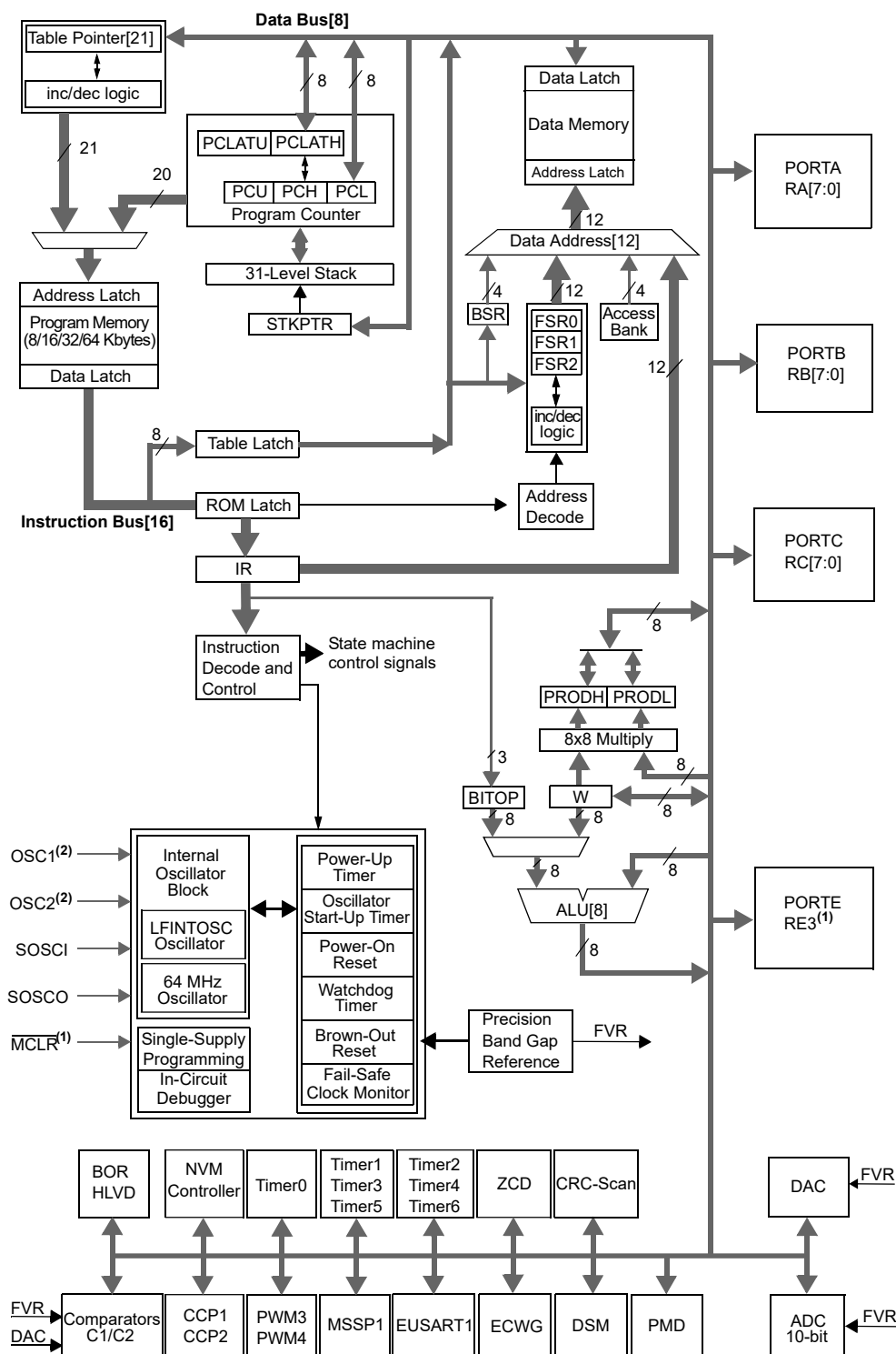
Figure 2-1. PIC18F24/25Q10 Family Block Diagram
