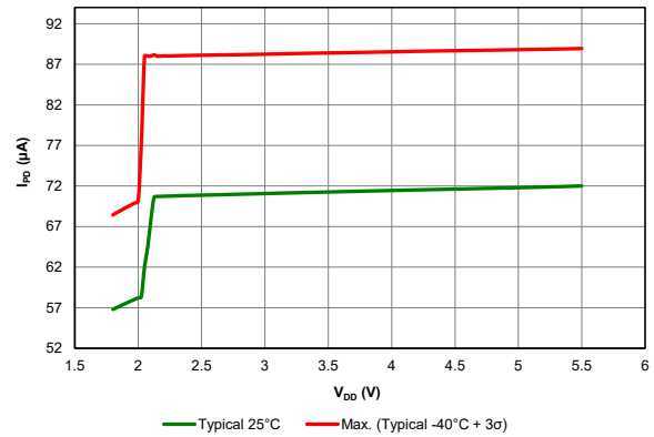
Figure 39-50. I_{PD} Base (VREGPM = 01)
