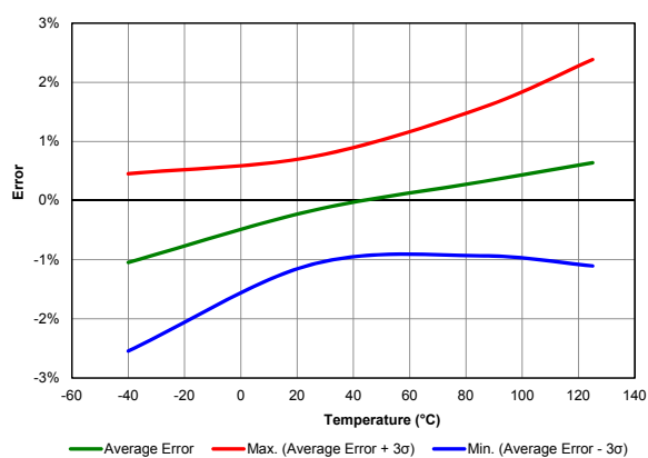
Figure 39-31. FVR Voltage Error 4x ( V_{DD} = 5.5\text{ V} )
