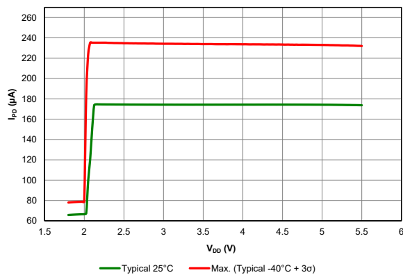
Figure 39-51. I_{PD} Base (VREGPM = 00)
