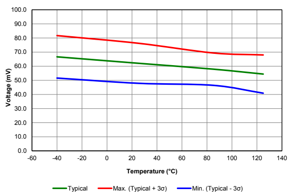
Figure 39-13. Brown-Out Reset Hysteresis, Trip Point (BORV = 00)
