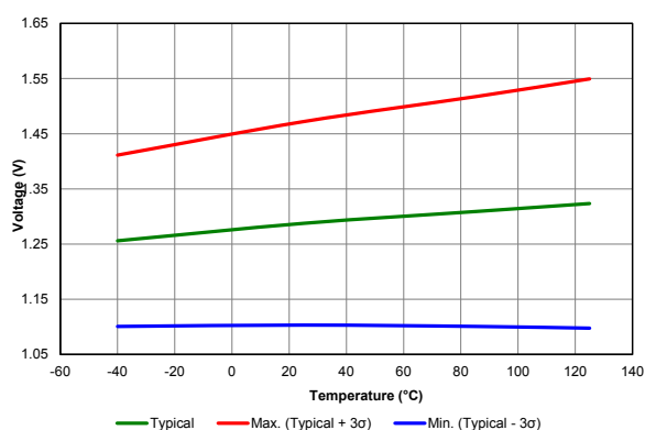
Figure 39-65. POR Rearm Voltage ( V_{REGPM} = 1\times )
