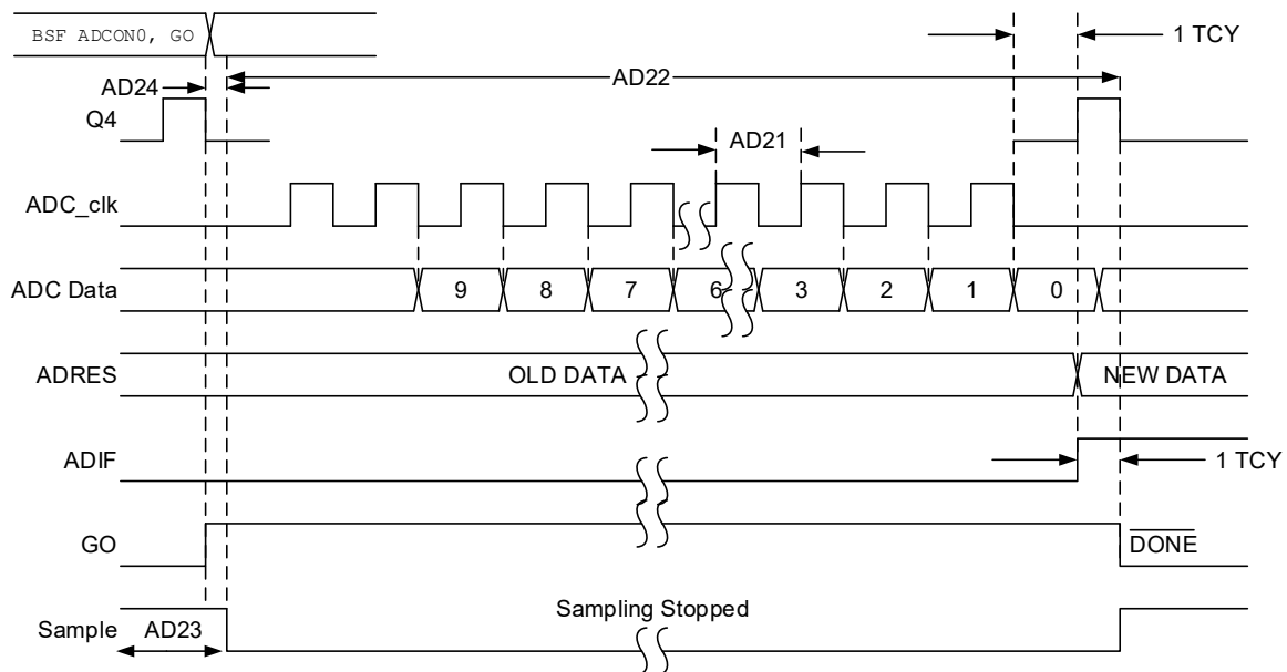
Figure 38-10. ADC Conversion Timing (ADC Clock from F_{RC} )
