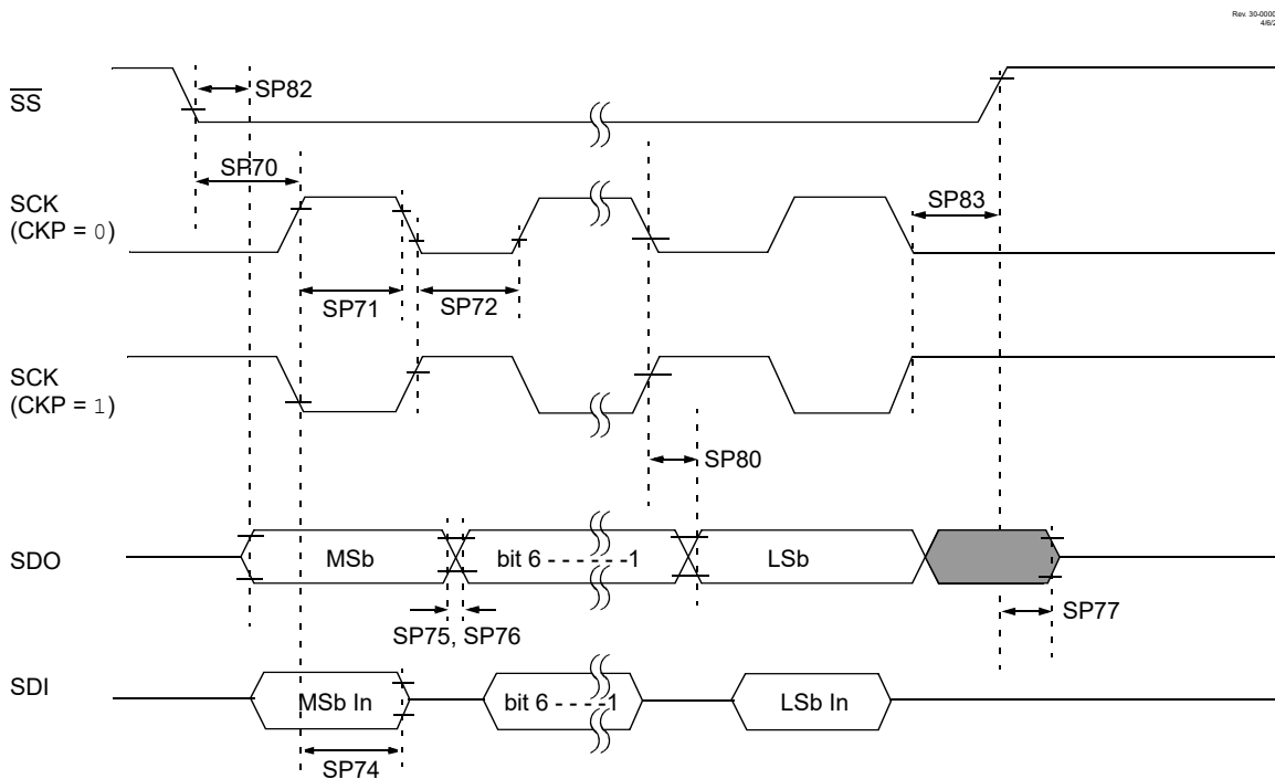
Figure 38-18. SPI Client Mode Timing (CKE = 1)
