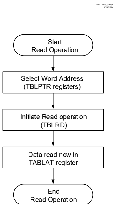
Figure 12-5. Program Flash Memory Read Flowchart
