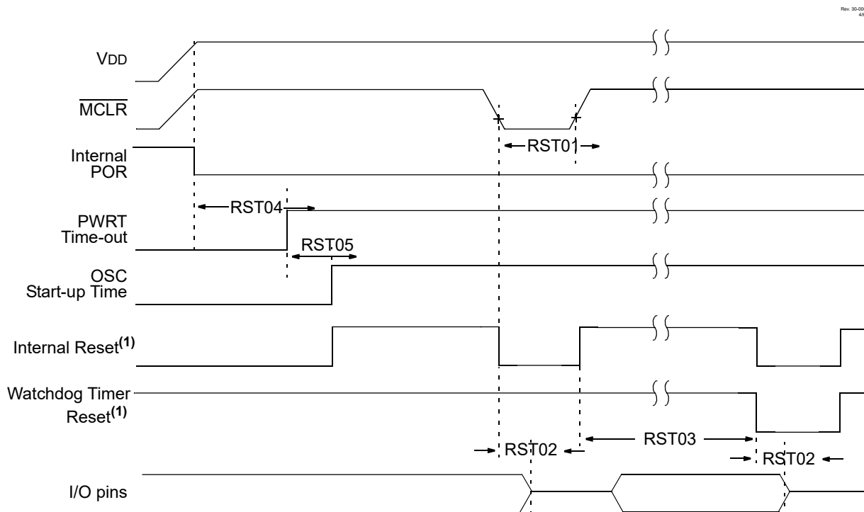
Figure 38-7. Reset, Watchdog Timer, Oscillator Start-up Time and Power-up Timer Timing
