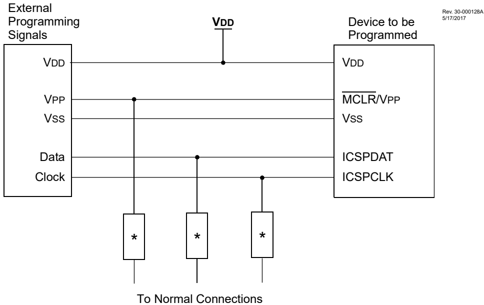
Figure 36-3. Typical Connection for ICSP™ Programming
