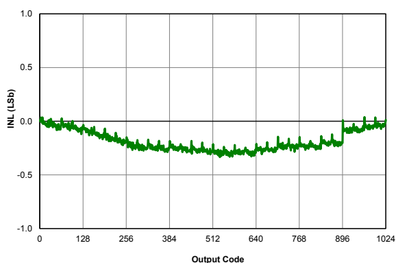
Figure 39-5. ADC, INL, V_{DD} = 3.0V , T_{AD} = 1 \mu s , 25^{\circ}C
