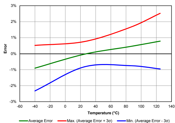
Figure 39-30. FVR Voltage Error 2x ( V_{DD} = 5.5\text{ V} )
