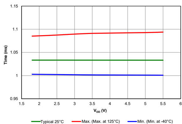
Figure 39-82. WDT Base Time-Out Period (WDTPS = 0)
