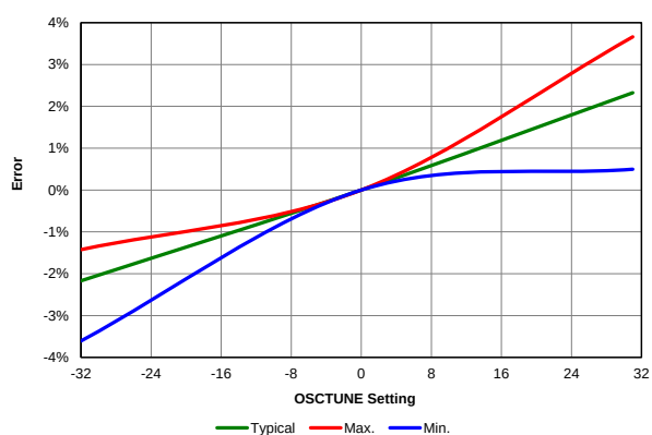
Figure 39-62. OSCTUNE Frequency Range (Normalized to Center Frequency)
