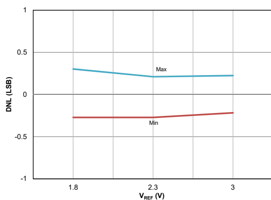
Figure 39-9. ADC 10-bit, DNL, V_{DD} = 3.0V , T_{AD} = 1 \mu s , Min and Max values at 125^{\circ}C + 3\sigma
