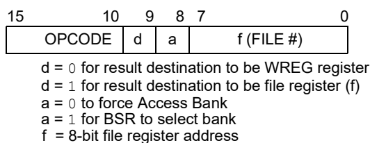
Figure 37-1. General Format for Instructions
