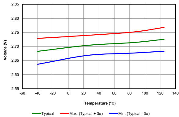
Figure 39-14. Brown-Out Reset Voltage, Trip Point (BORV = 01)
