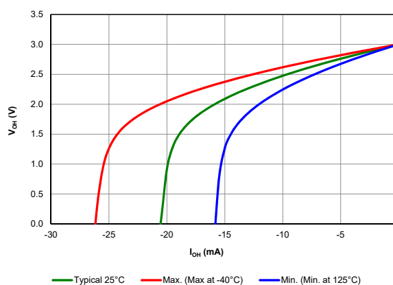
Figure 39-77. V_{OH} vs. I_{OH} over Temperature, V_{DD} = 3V
