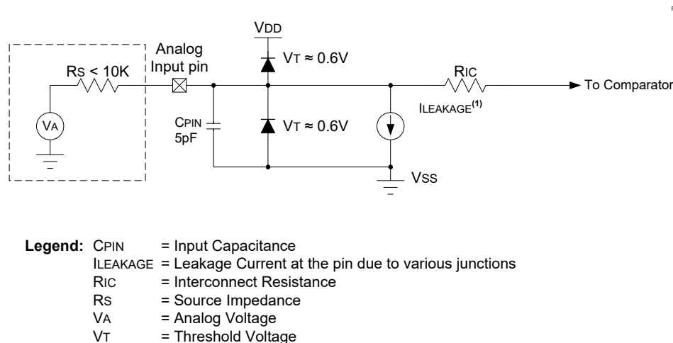
Figure 33-3. Analog Input Model
