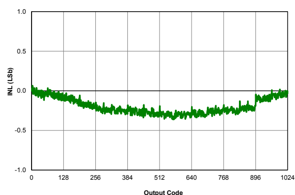
Figure 39-6. ADC, INL, V_{DD} = 3.0V , T_{AD} = 4 \mu s , 25^{\circ}C
