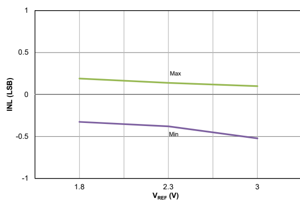
Figure 39-10. ADC 10-BIT, INL, V_{DD} = 3.0V , T_{AD} = 1 \mu s , Min and Max values at 125^{\circ}C + 3\sigma
