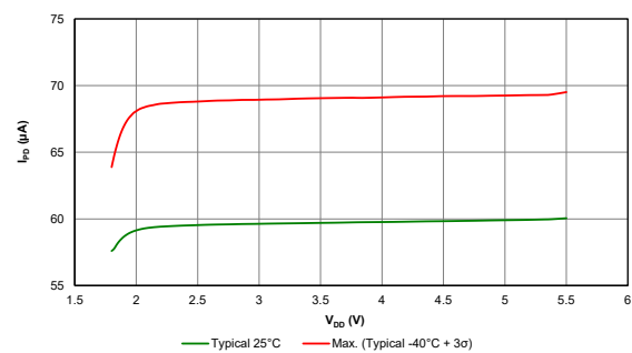
Figure 39-46. I PD , Comparator
