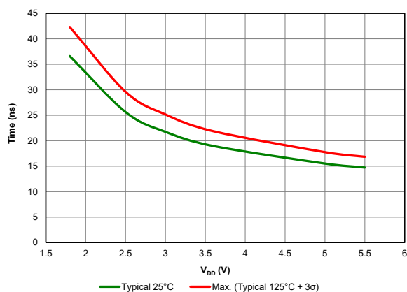
Figure 39-32. Rise Time, Slew Rate Control Enabled
