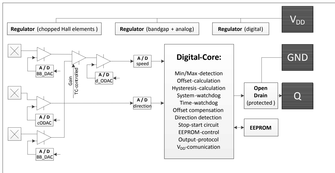
Figure 4 Block Diagram
