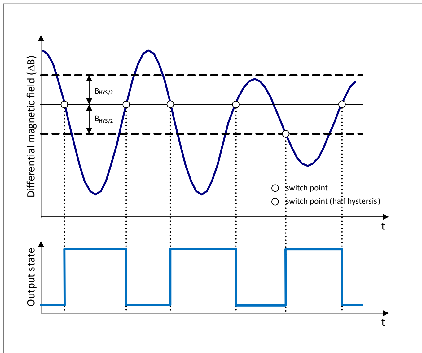
Figure 9 Hidden Hysteresis in protocol-variant without direction detection
