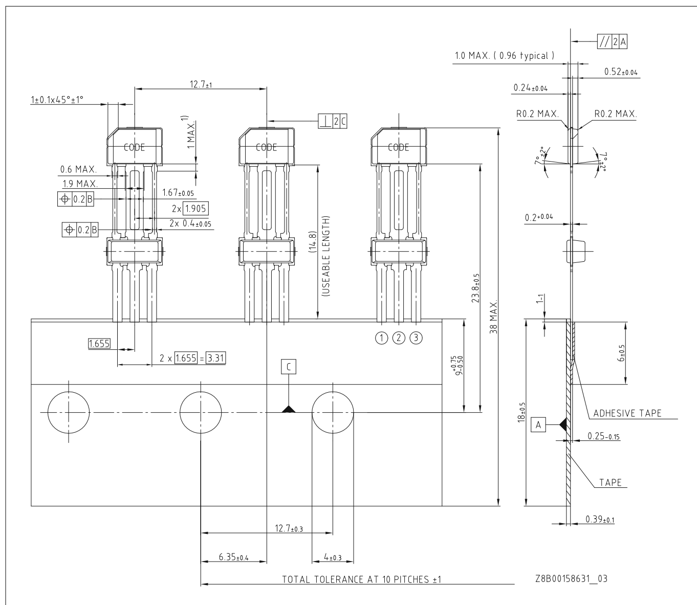
Figure 22 PG-SSO-3-5x Ammopack
