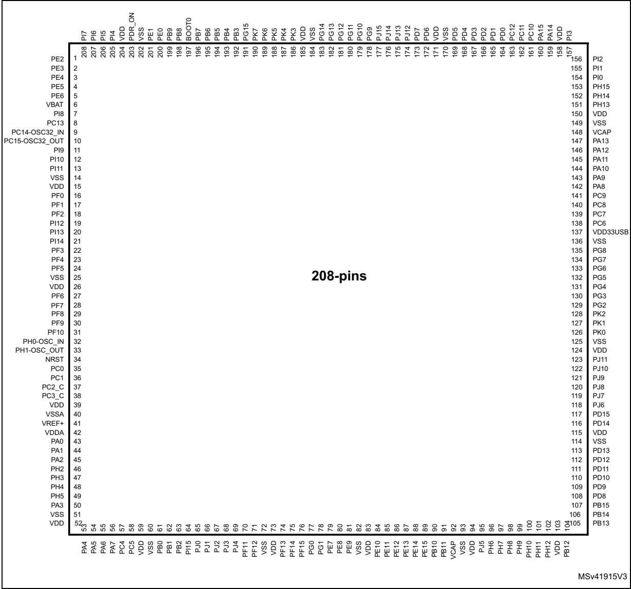
Figure 11. LQFP208 pinout
