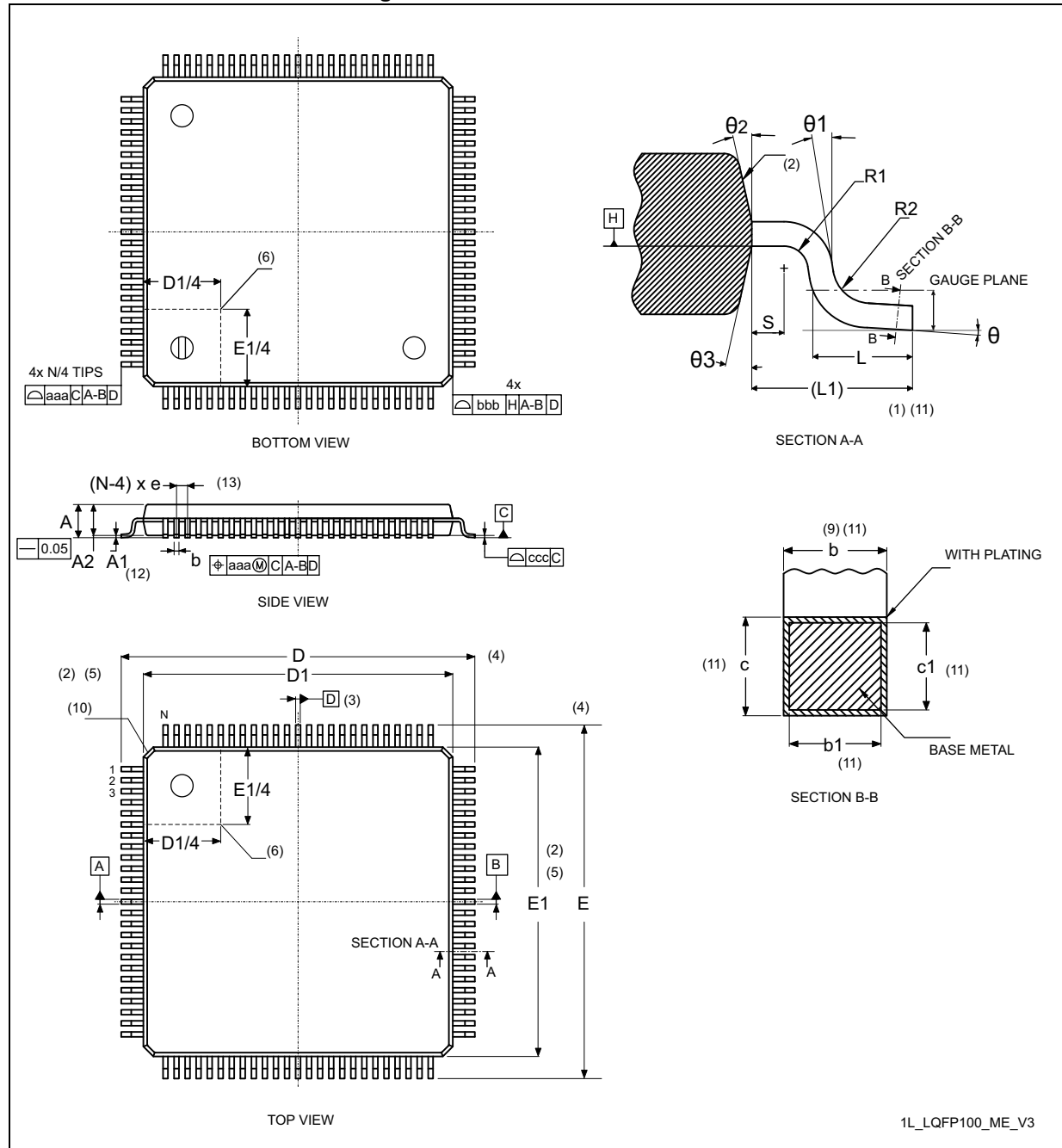
Figure 120. LQFP100 - Outline (15)
