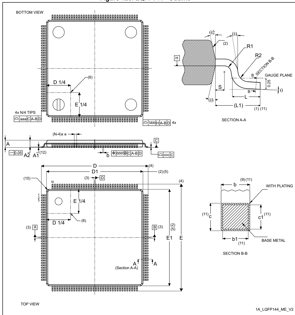
Figure 126. LQFP144 - Outline (15)
